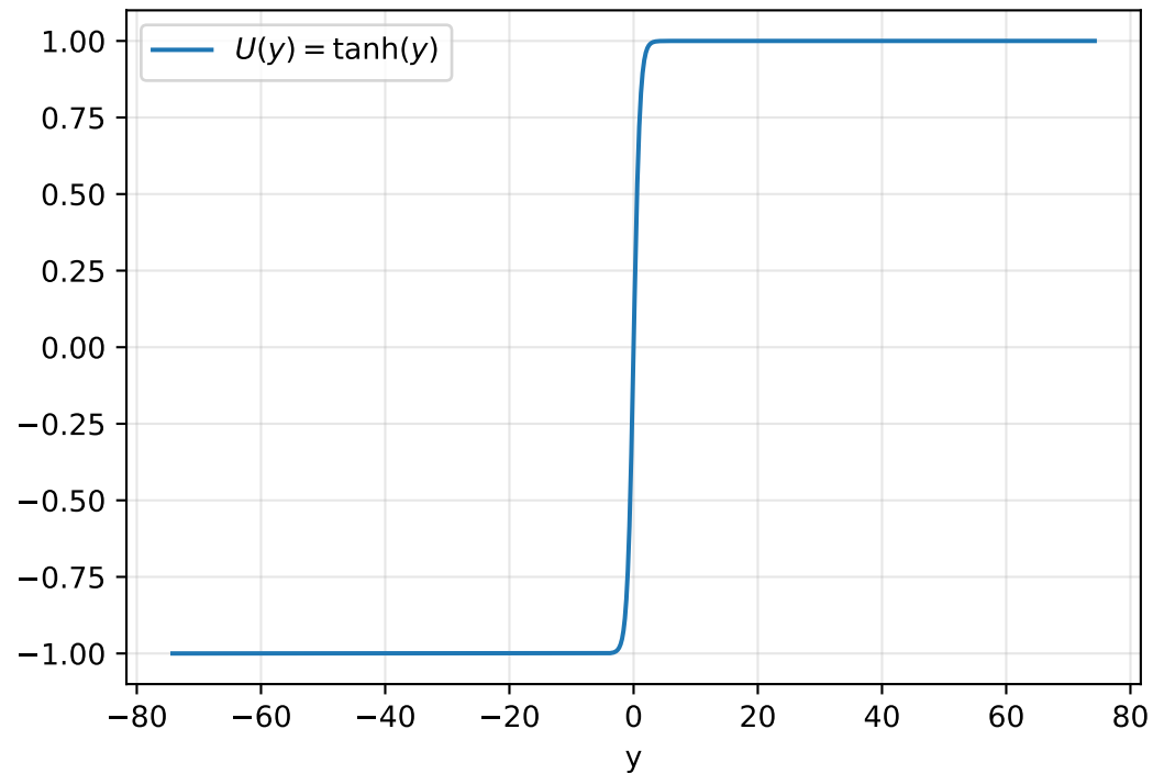
c_i^{PINN} = 0.04315 , c_i^{ref} = 0.04427
