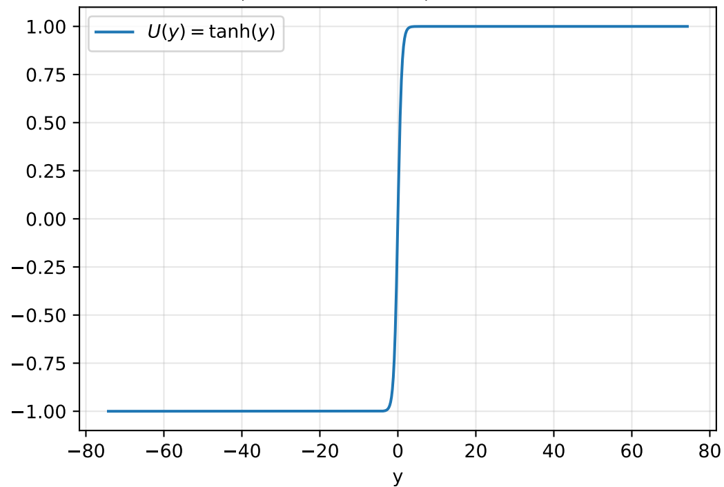
c_i^{PINN} = 0.33252 , c_i^{ref} = 0.33292
