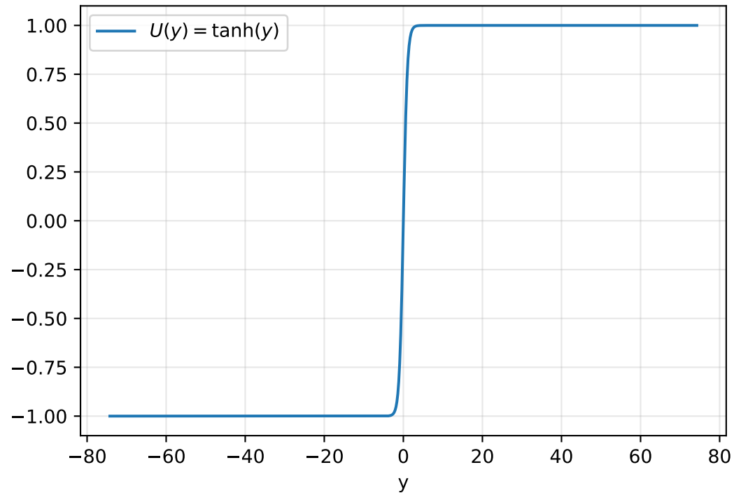
c_i^{PINN} = 0.02626 , c_i^{ref} = 0.00999
