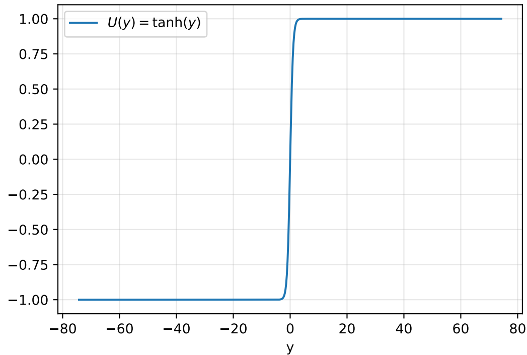
c_i^{PINN} = 0.15998 , c_i^{ref} = 0.15968
