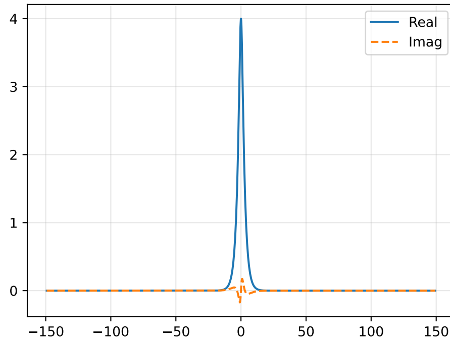
Pressure Perturbation \hat{p}
