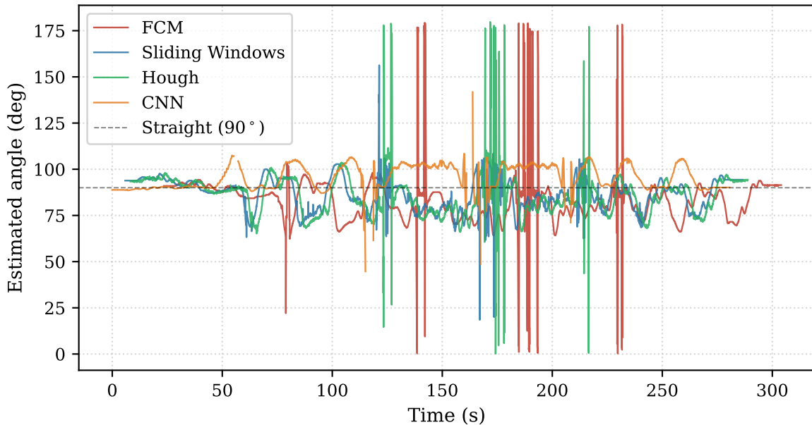
Lane heading estimate over time
