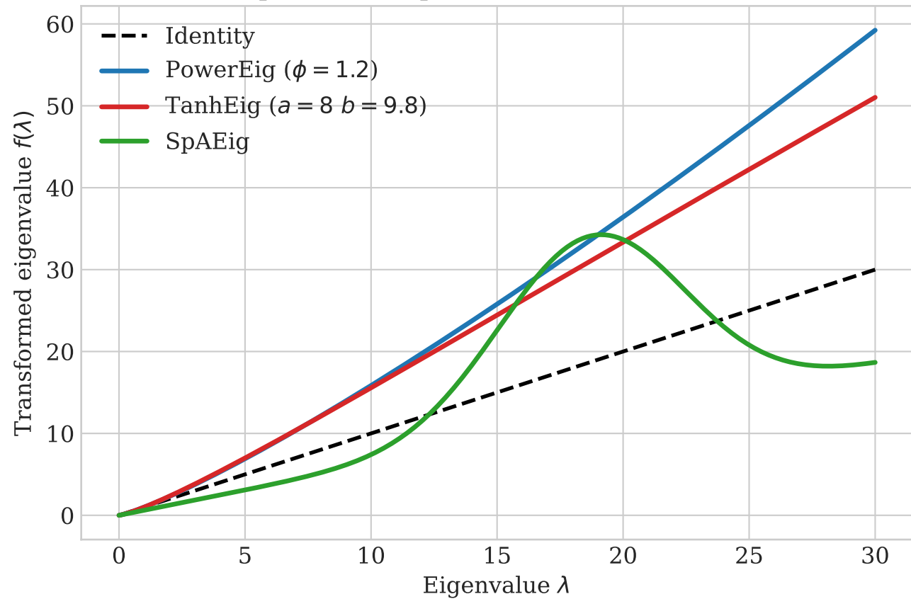
Comparison of spectral activation functions
