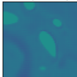
Pred. probability
