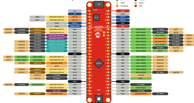
On-Board Peripherals
