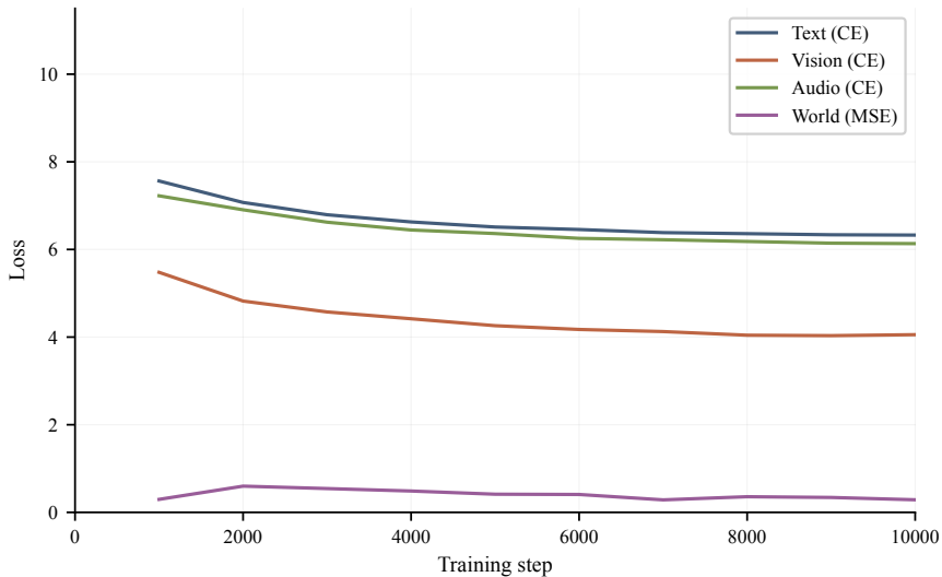
Quatrix-60m multimodal: per-modality training loss
