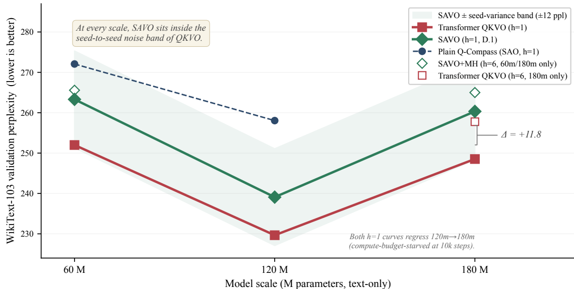
Text-LM scaling: SAVO tracks rank-matched QKVO across three scales
