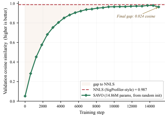
Phase 1: SAVO approaches NNLS signature decomposition
