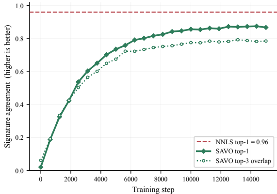
Top-k signature agreement
