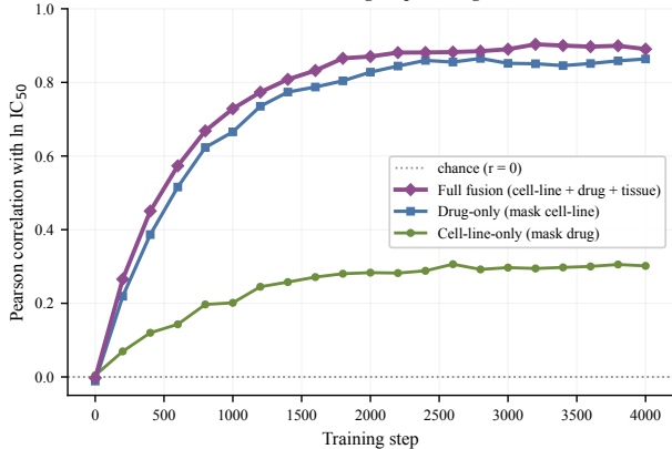
Phase 3: GDSC drug-response regression
