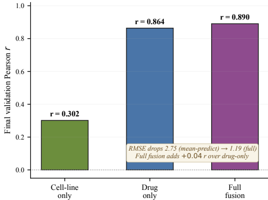
Channel ablation at final step
