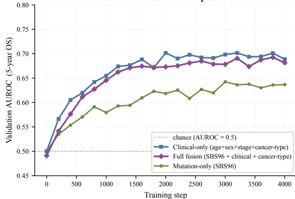
Phase 4: multimodal survival prediction
