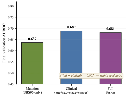
Channel ablation at final step
