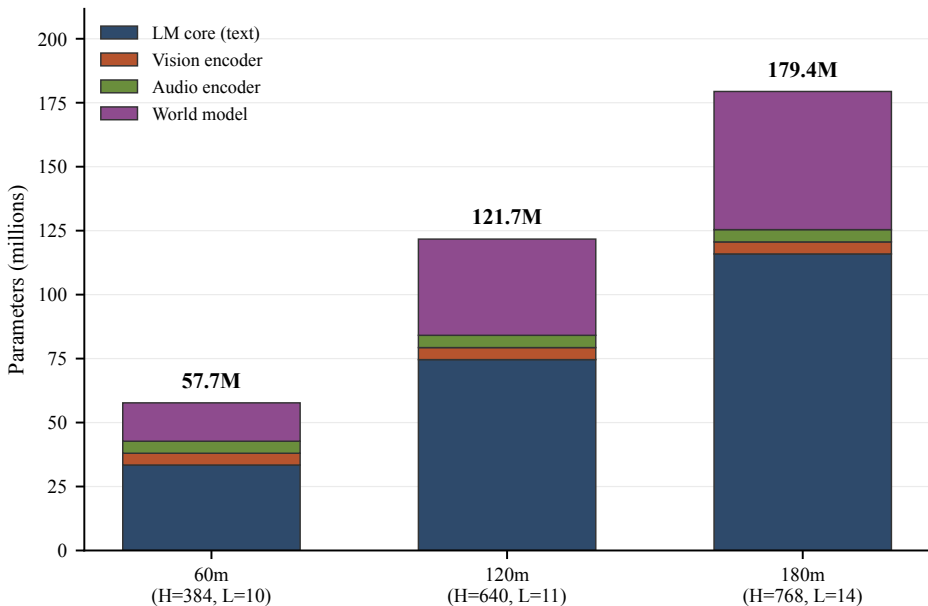
Parameter breakdown across three Quatrix scales
