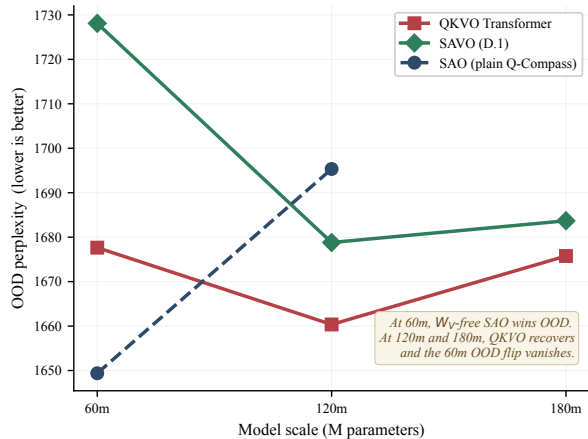
b. Out-of-distribution perplexity (arxiv + pubmed avg)
