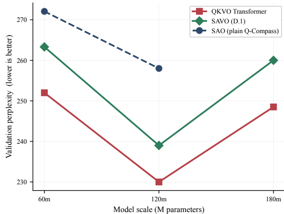
a. In-distribution perplexity (WT-103 val)
