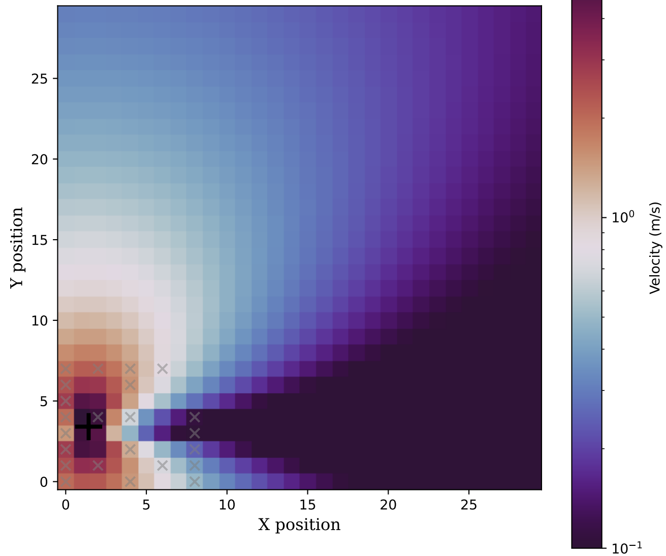
Fitted Lamb-Oseen
