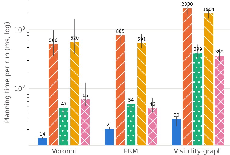
(b) Planning compute (median, IQR)
