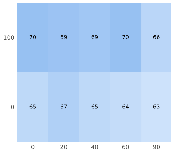
Visibility graph
