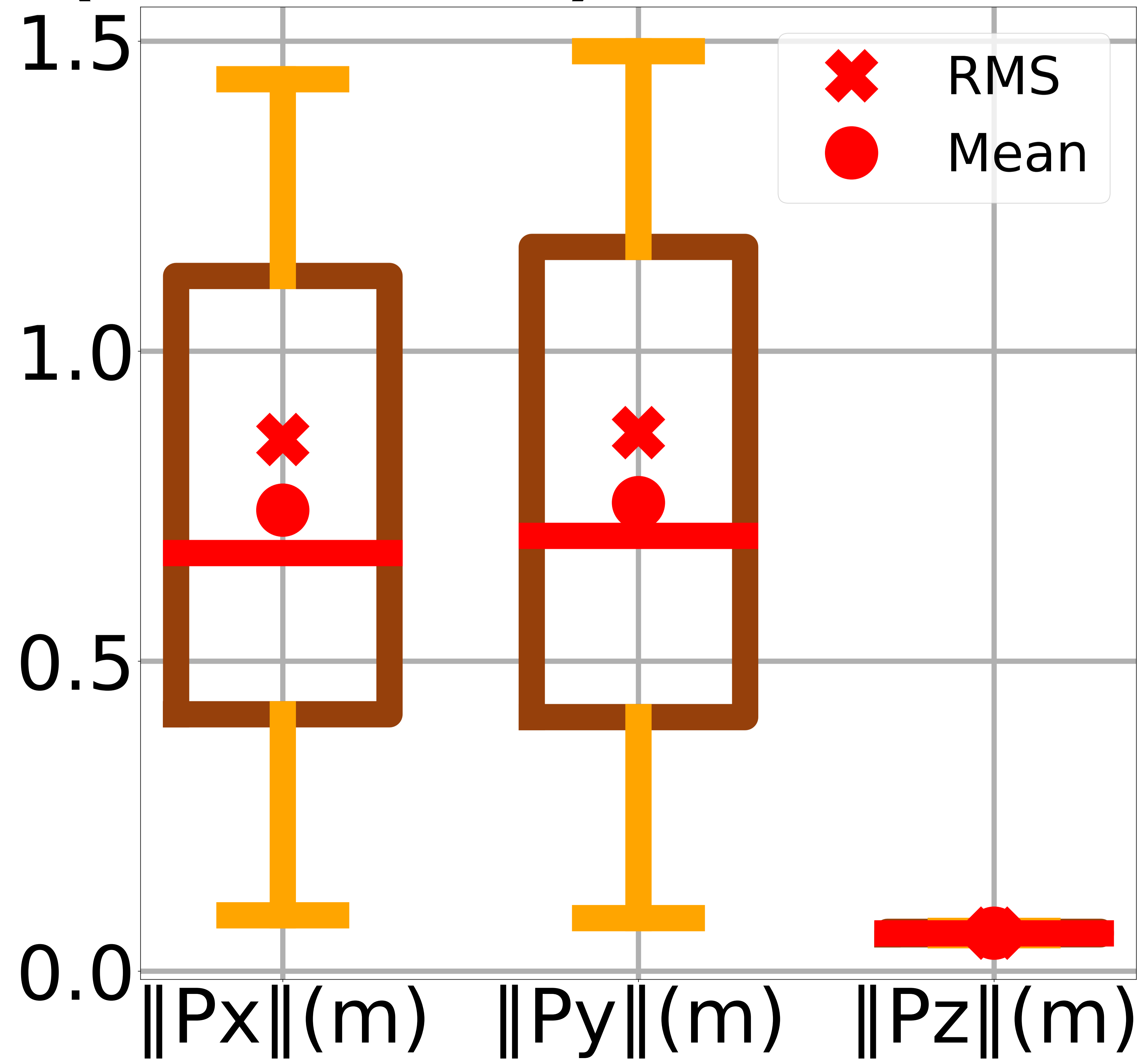
Long-1.0m/s-Fan (DFBC+INDI)-Position Error
