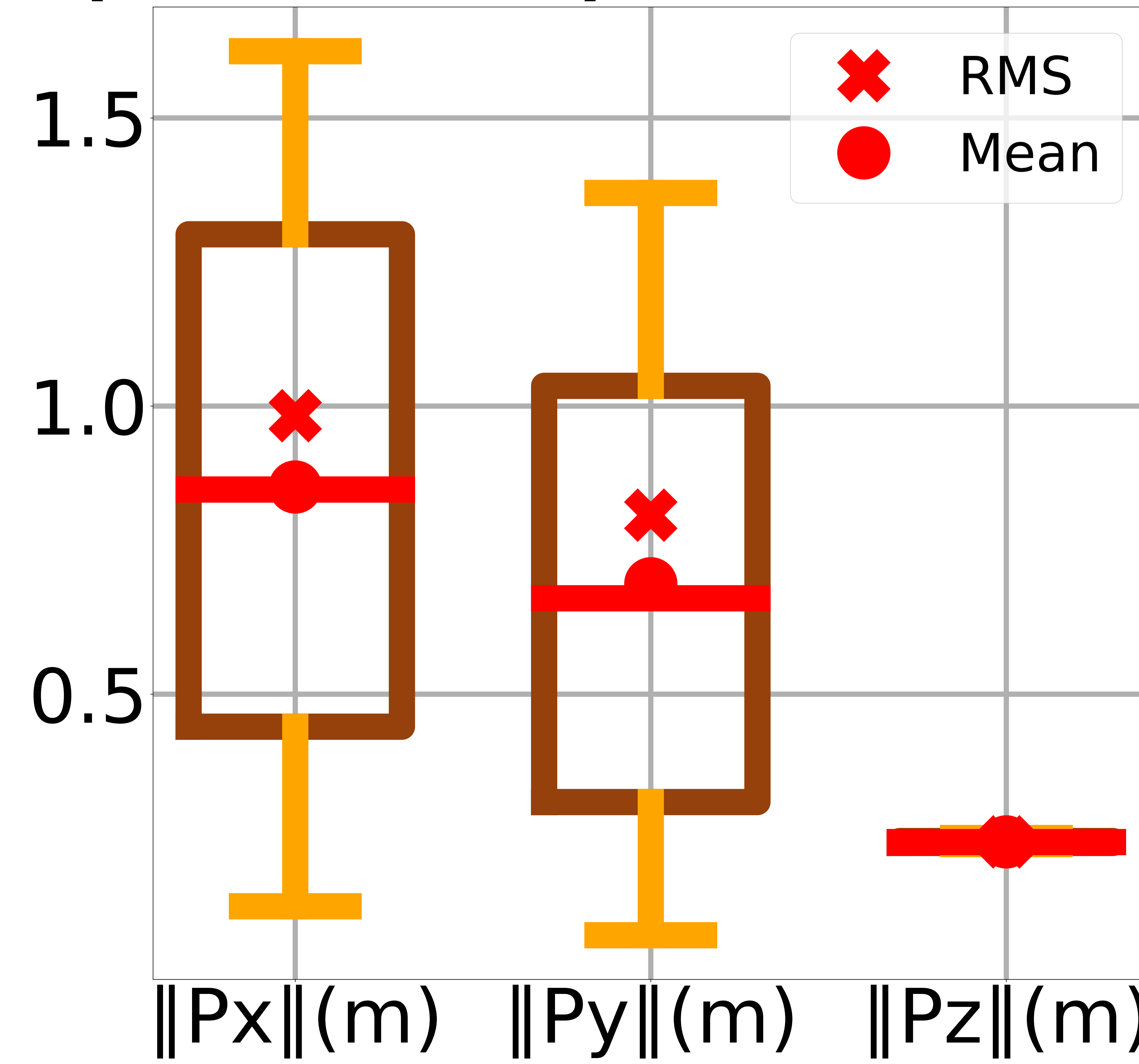
Ultralight-0.4m/s-Payload (DFBC+INDI)-Position Error
