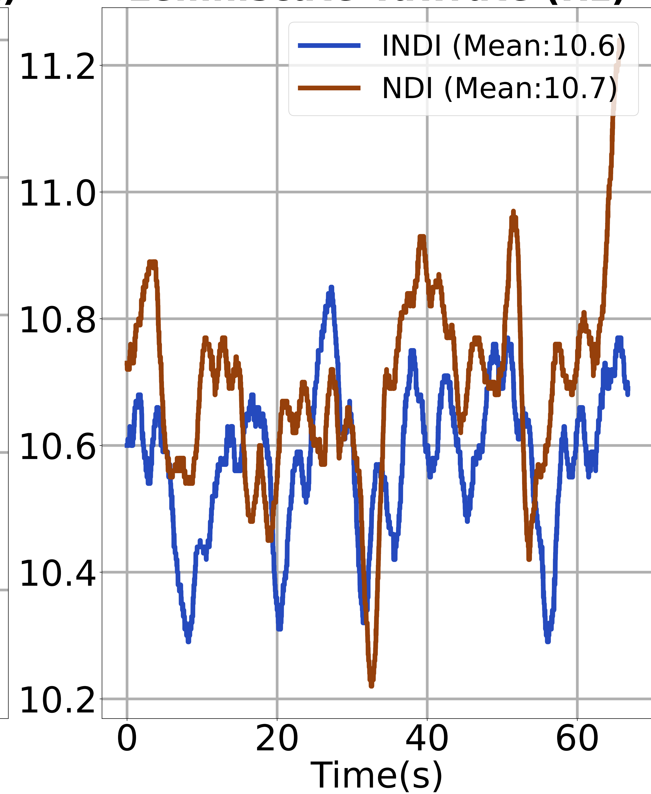
Lemniscate Yawrate (Hz)
