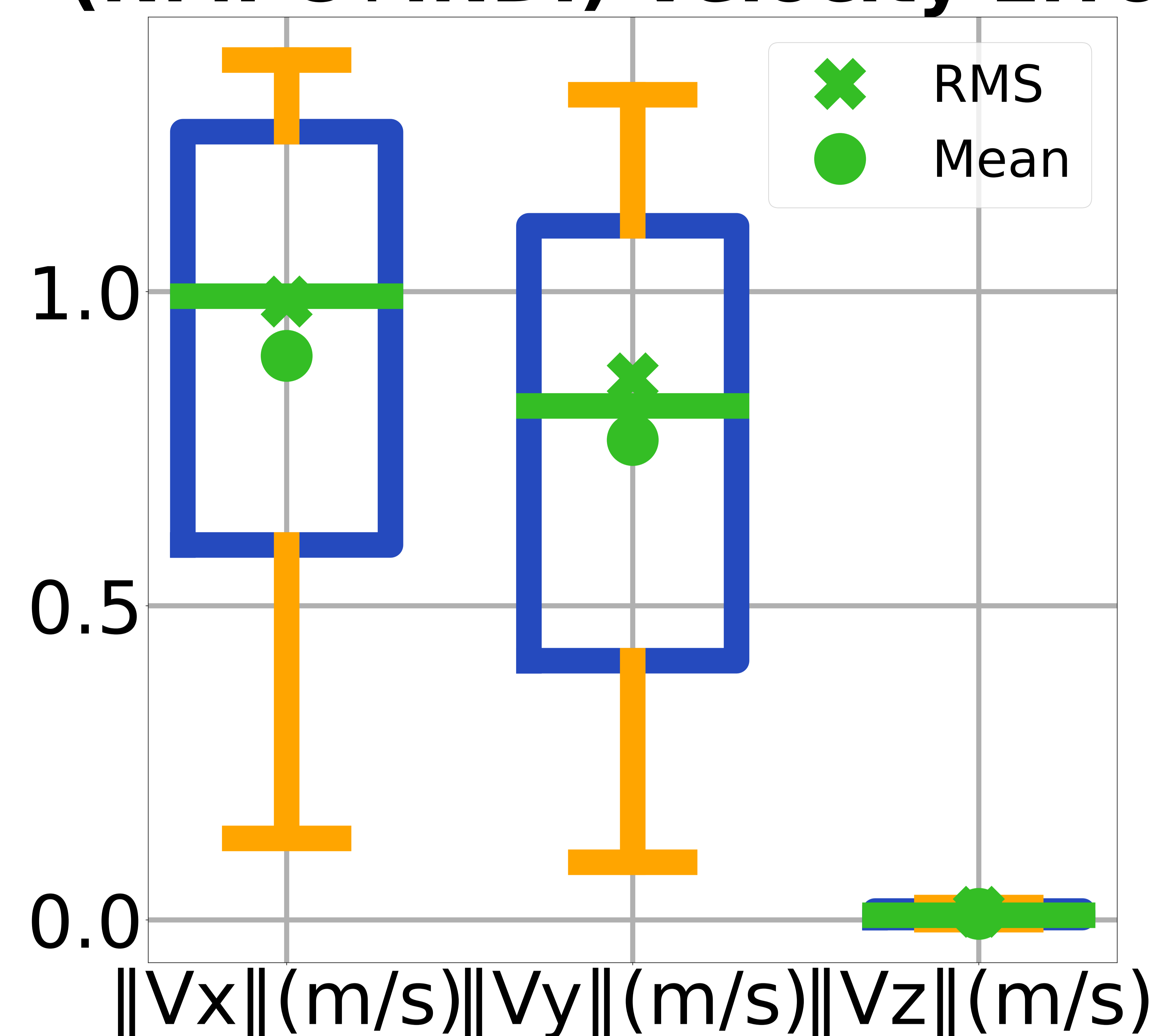
Long-1.0m/s-Fan (DFBC+INDI)-Velocity Error
