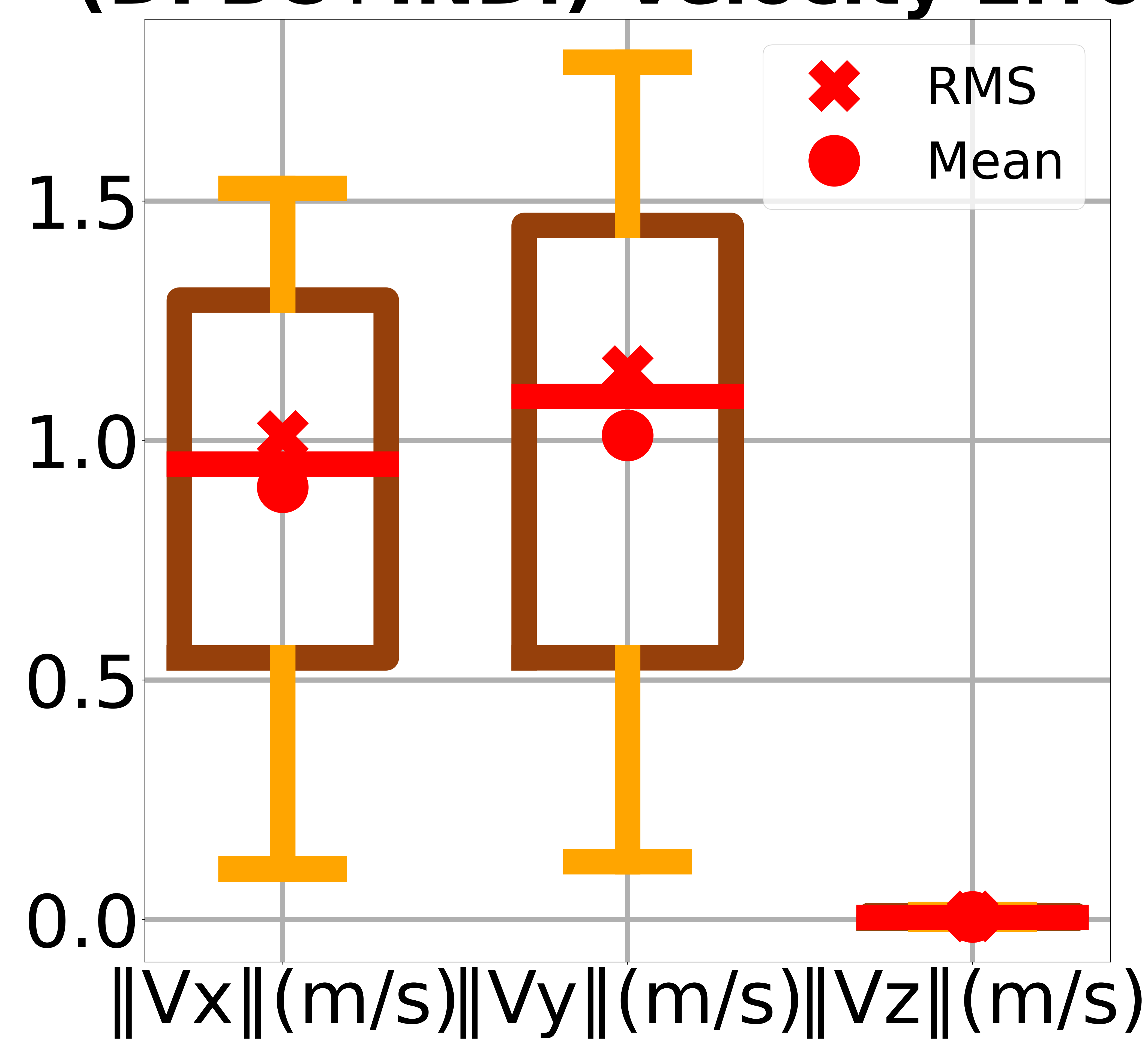
Short-1.0m/s-Fan (DFBC+INDI)-Velocity Error
