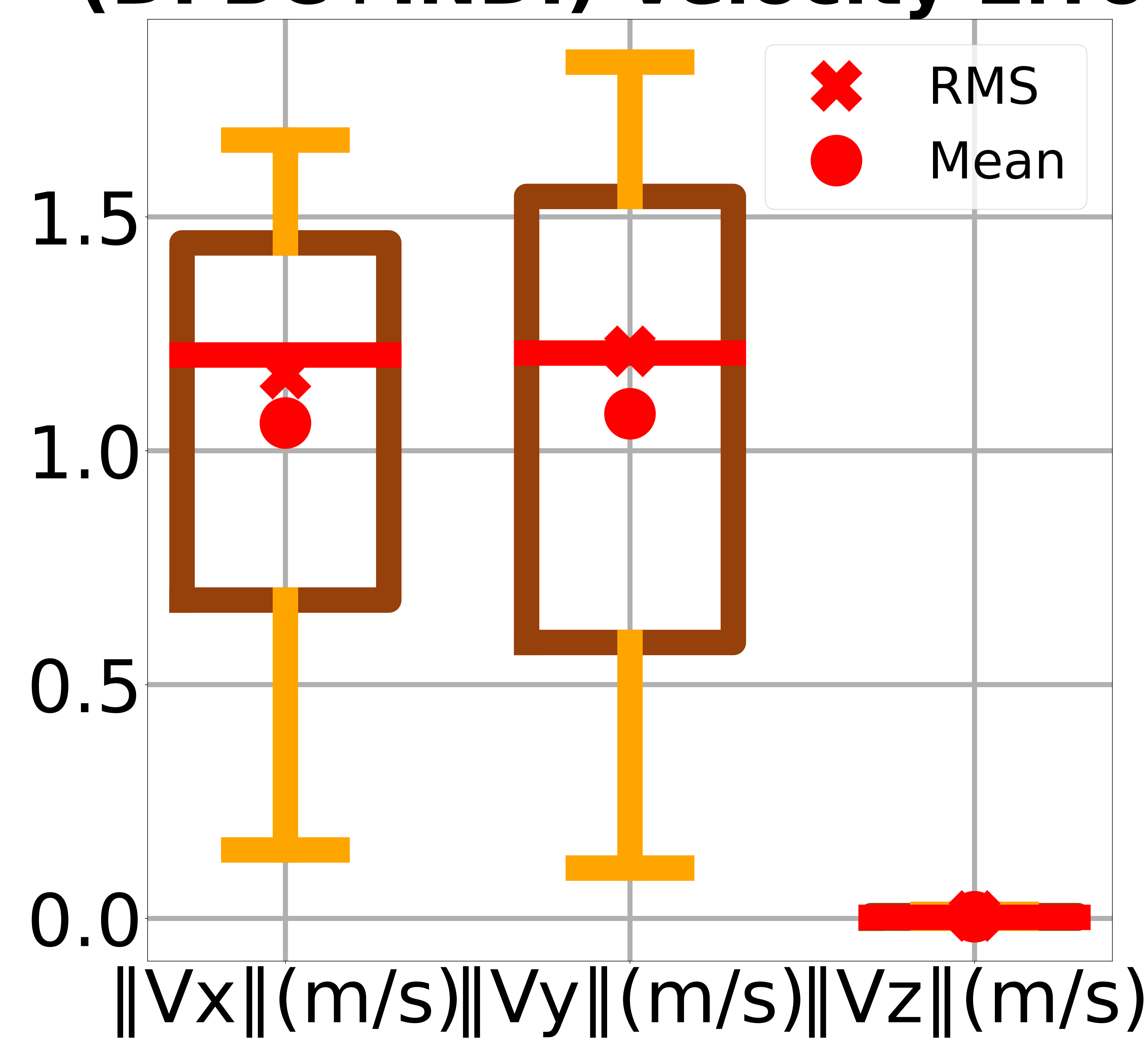
Long-1.0m/s-Fan (DFBC+INDI)-Velocity Error
