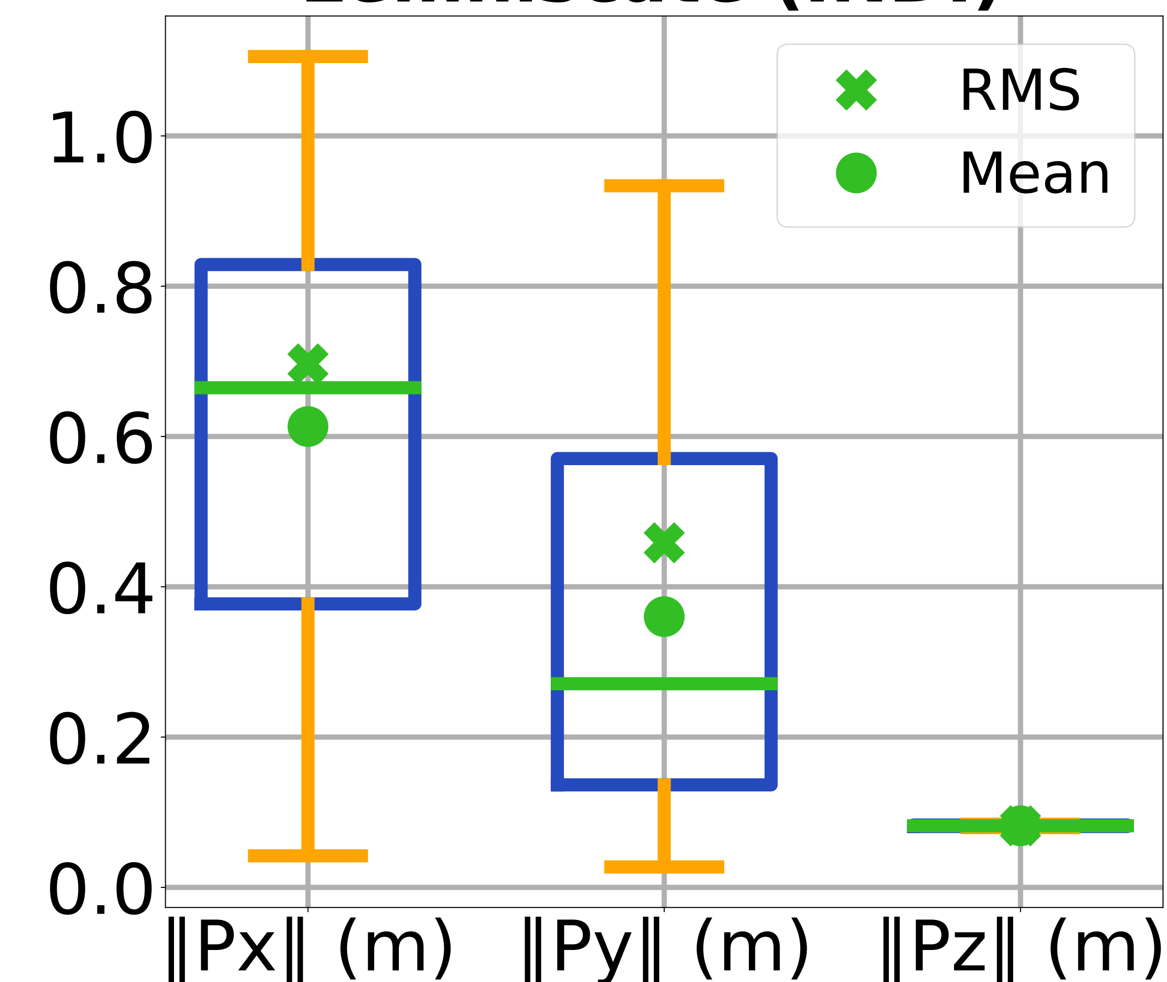
Lemniscate (INDI)
