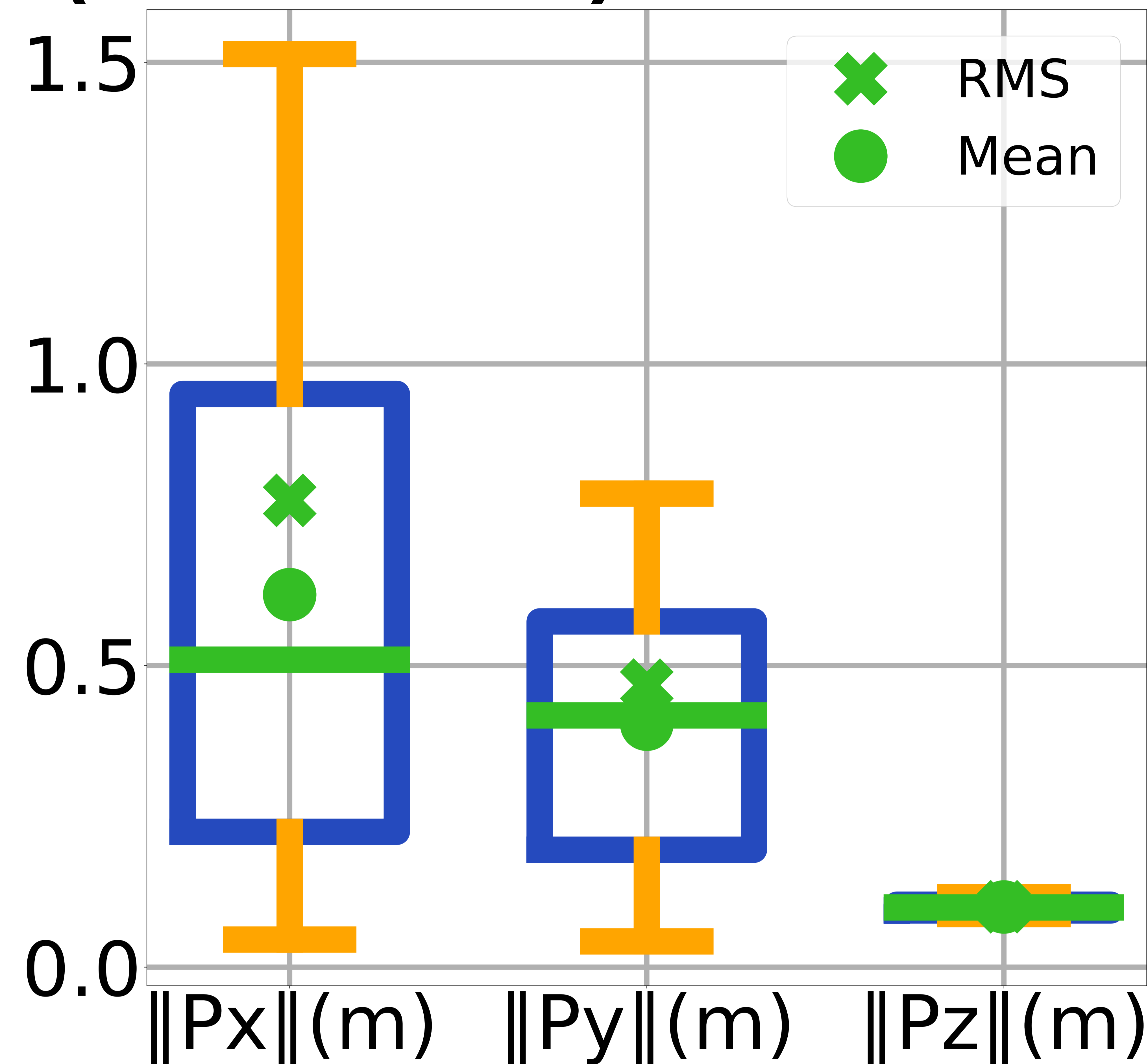
Short-1.0m/s-Fan (NMPC+INDI)-Position Error
