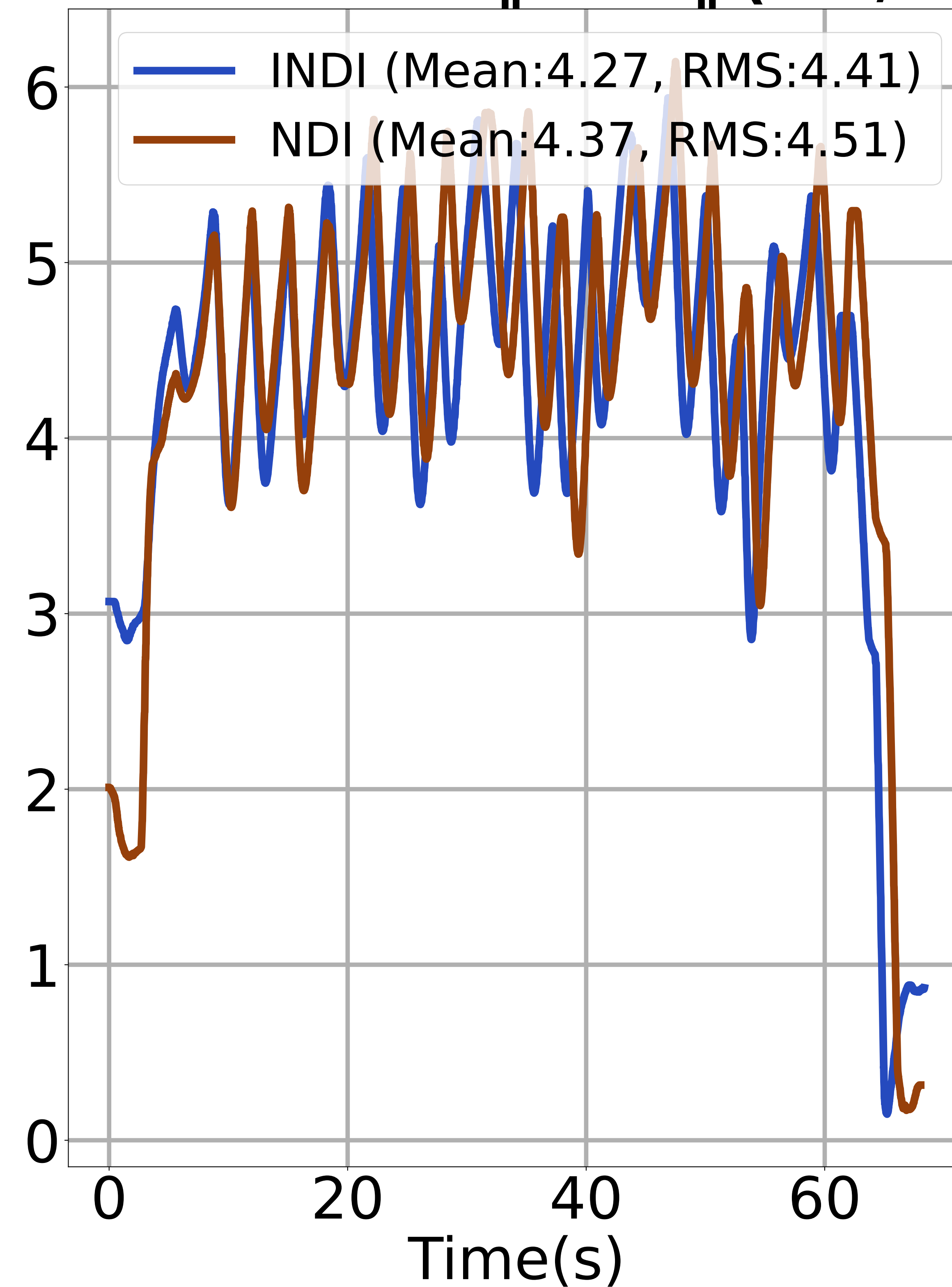
Elevated Circle \|\dot{\omega}DE\| (rad/s 2 )
