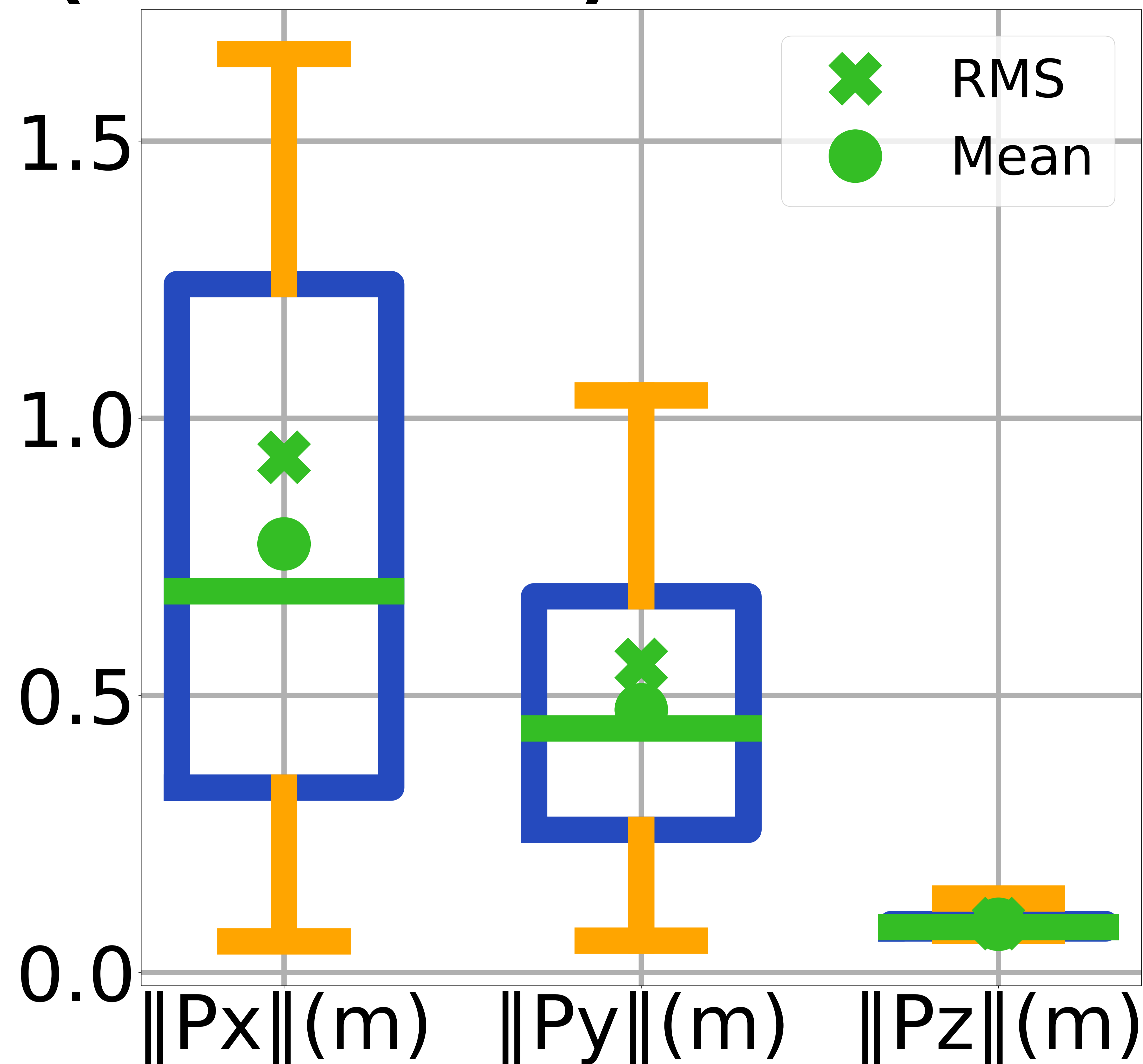
Long-1.0m/s-Fan (NMPC+INDI)-Position Error
