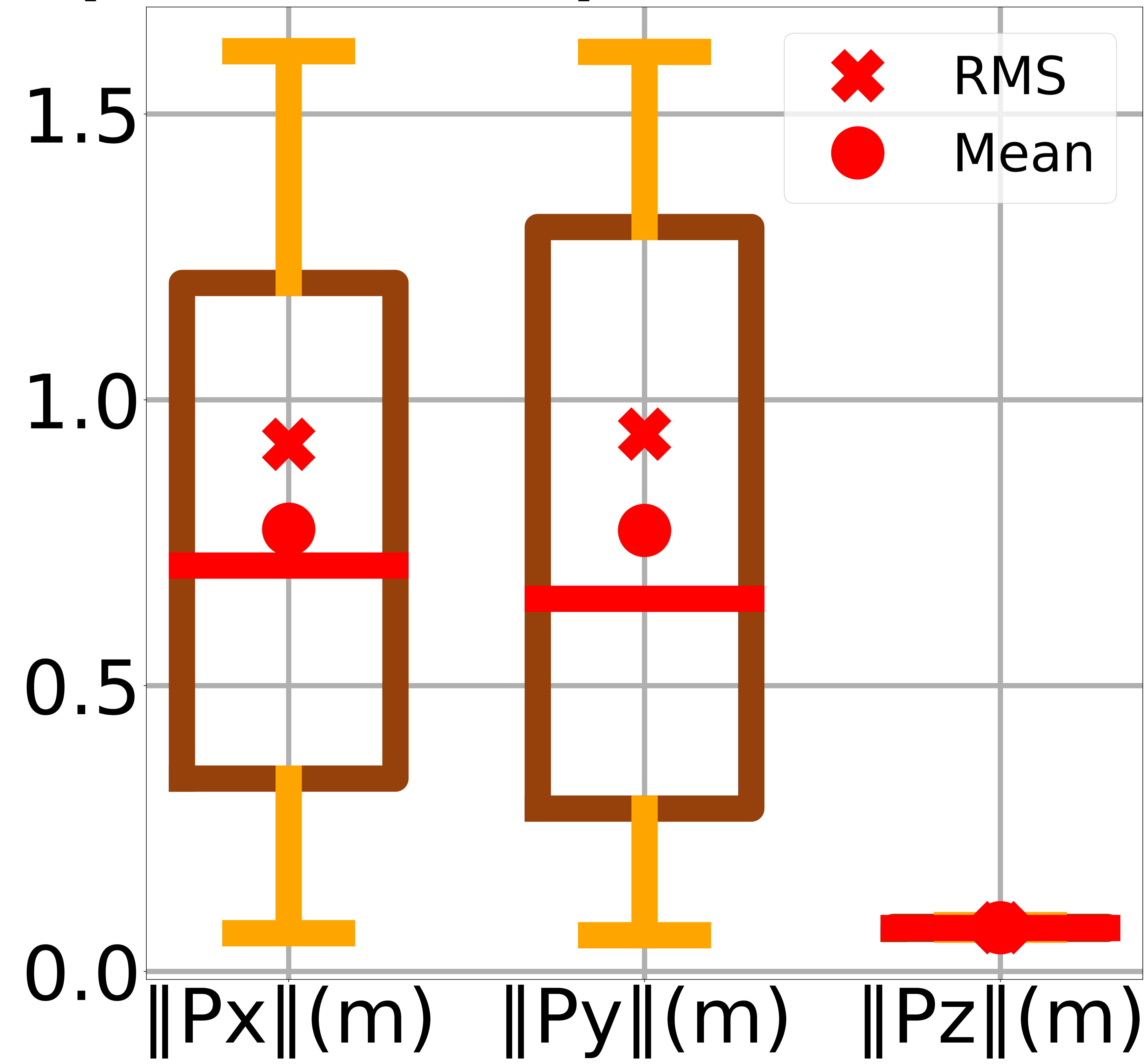
Short-1.0m/s-Fan (DFBC+INDI)-Position Error
