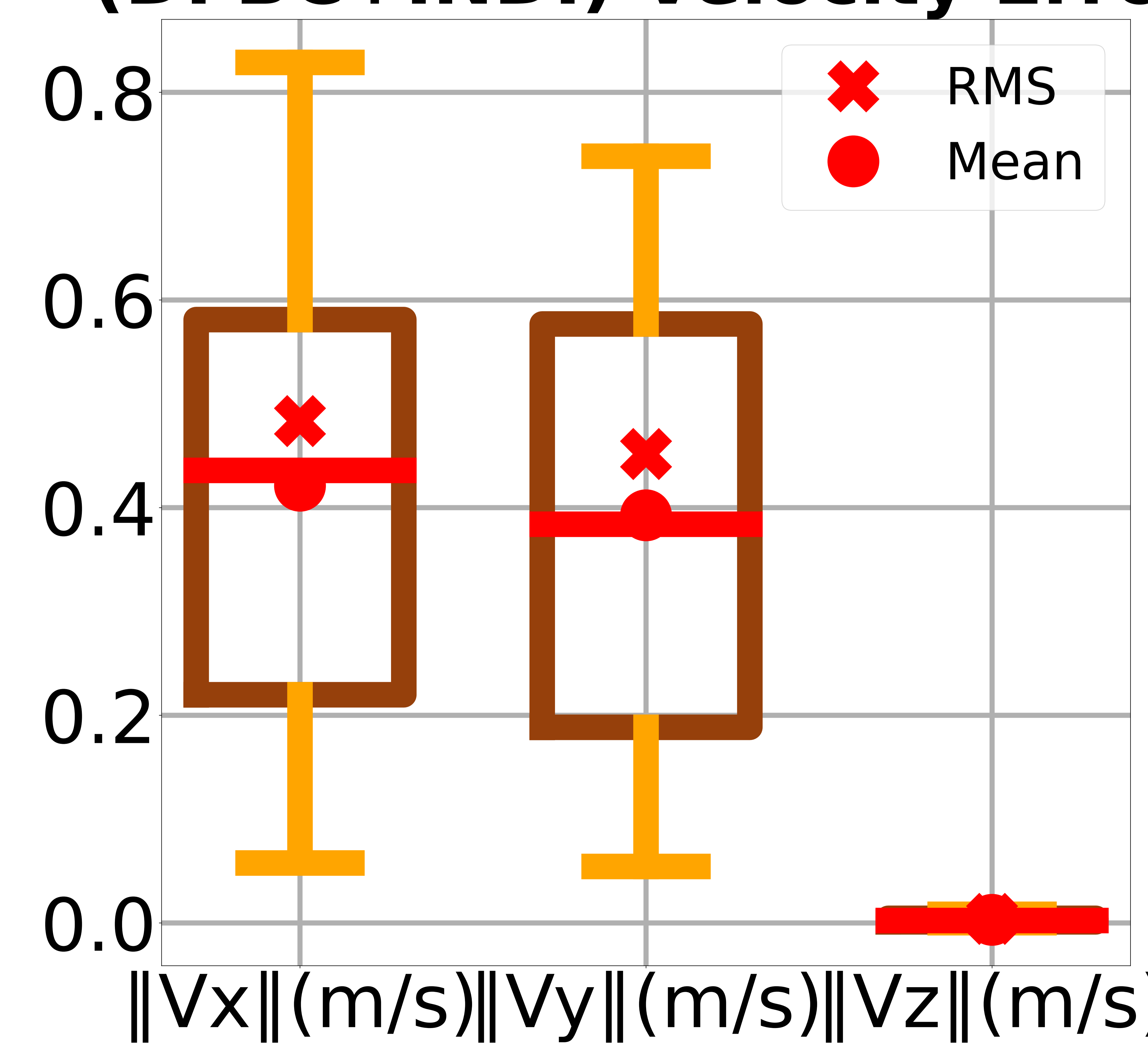
Ultralight-0.4m/s-Payload (DFBC+INDI)-Velocity Error
