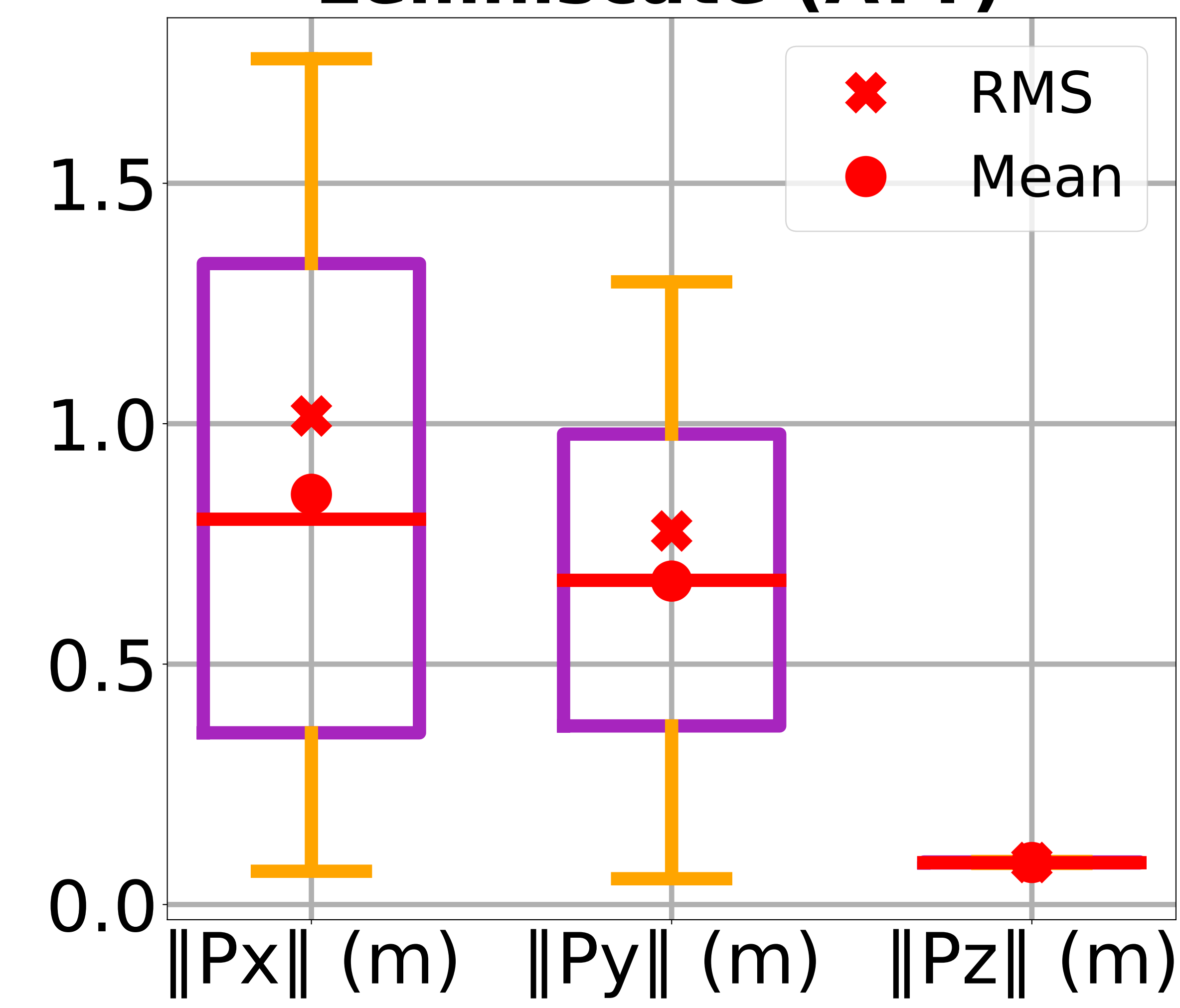
Lemniscate (ATT)
