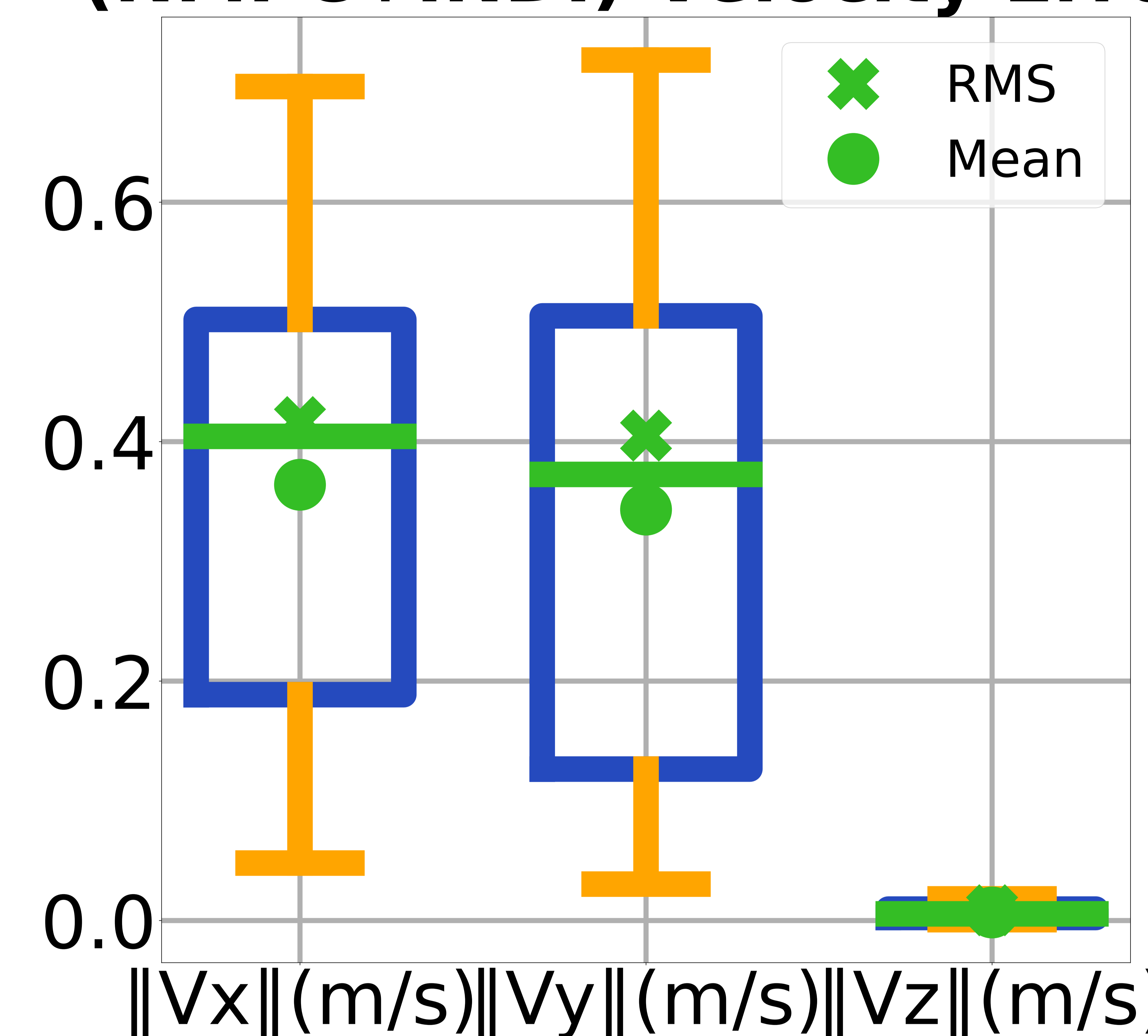
Ultralight-0.4m/s-Payload (DFBC+INDI)-Velocity Error
