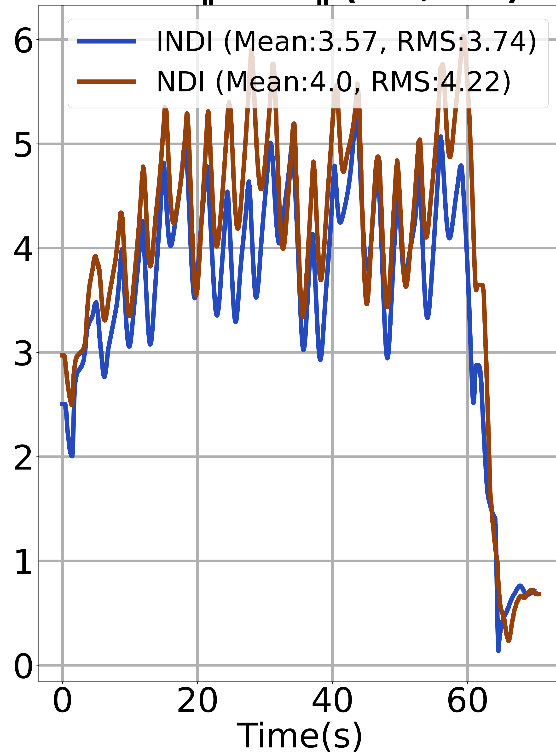
Circle \|\dot{\omega}DE\| (rad/s 2 )
