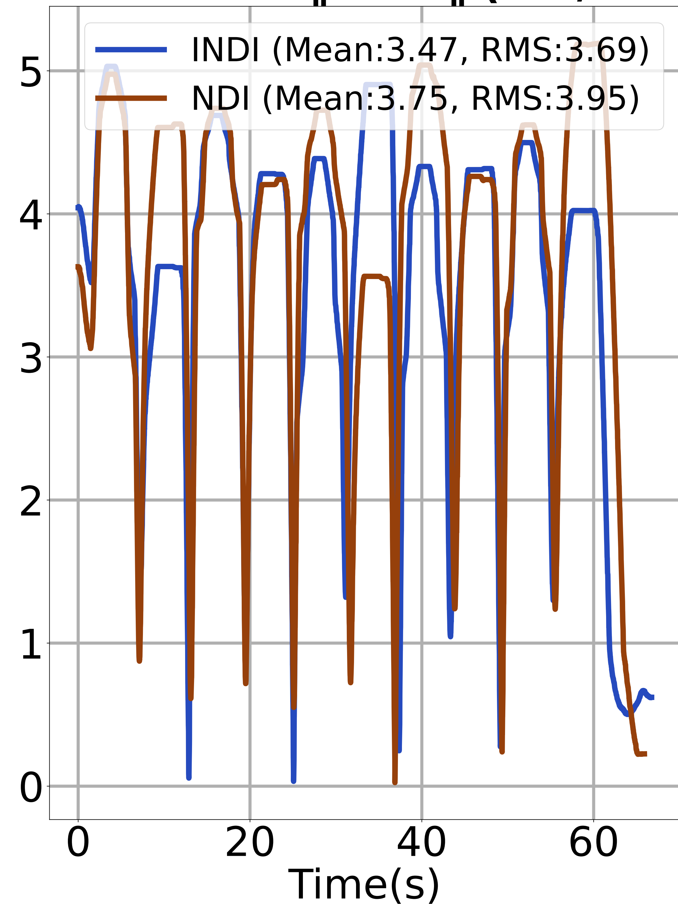
Lemniscate \|\dot{\omega}DE\| (rad/s 2 )
