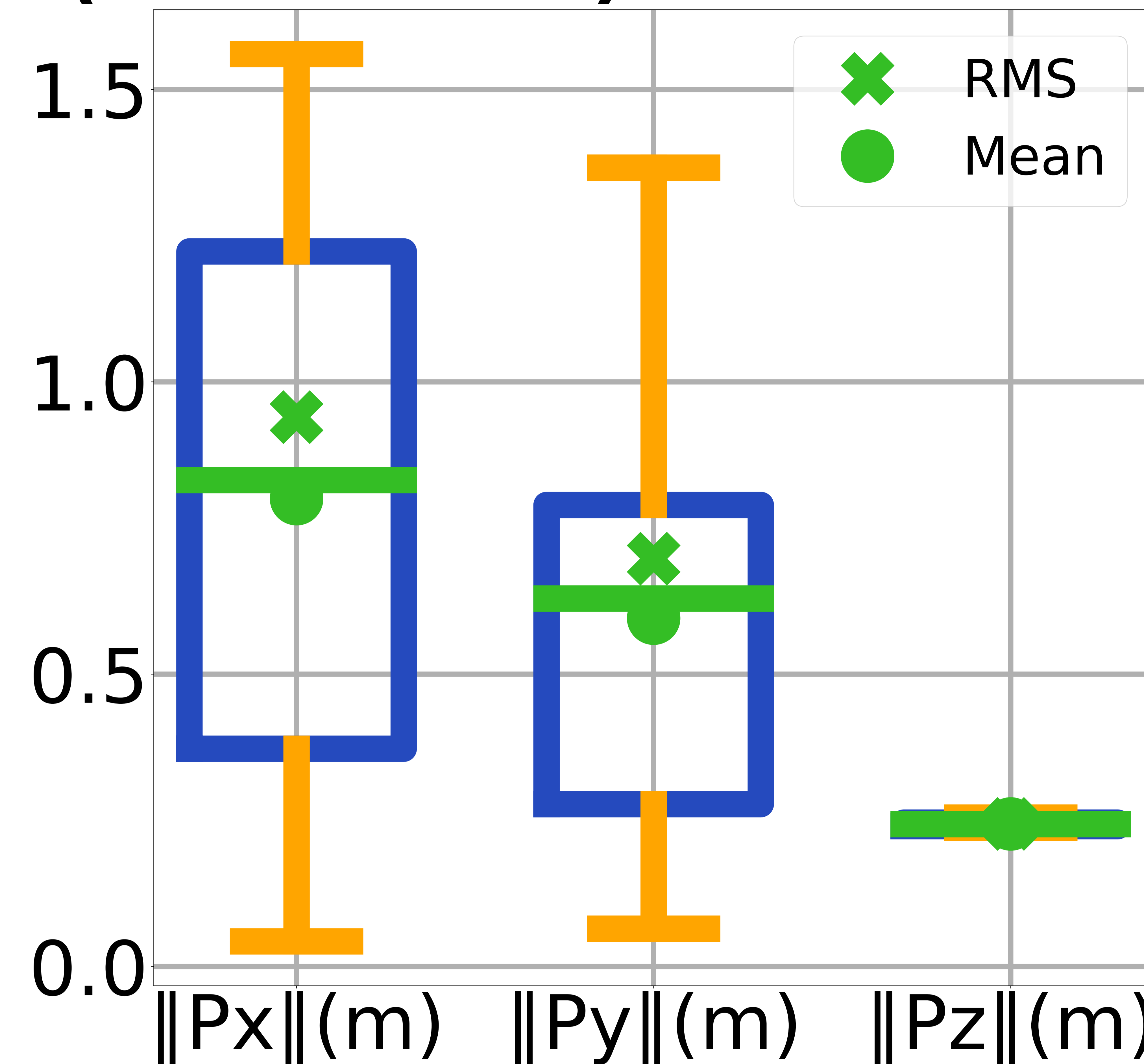
Ultralight-0.4m/s-Payload (NMPC+INDI)-Position Error
