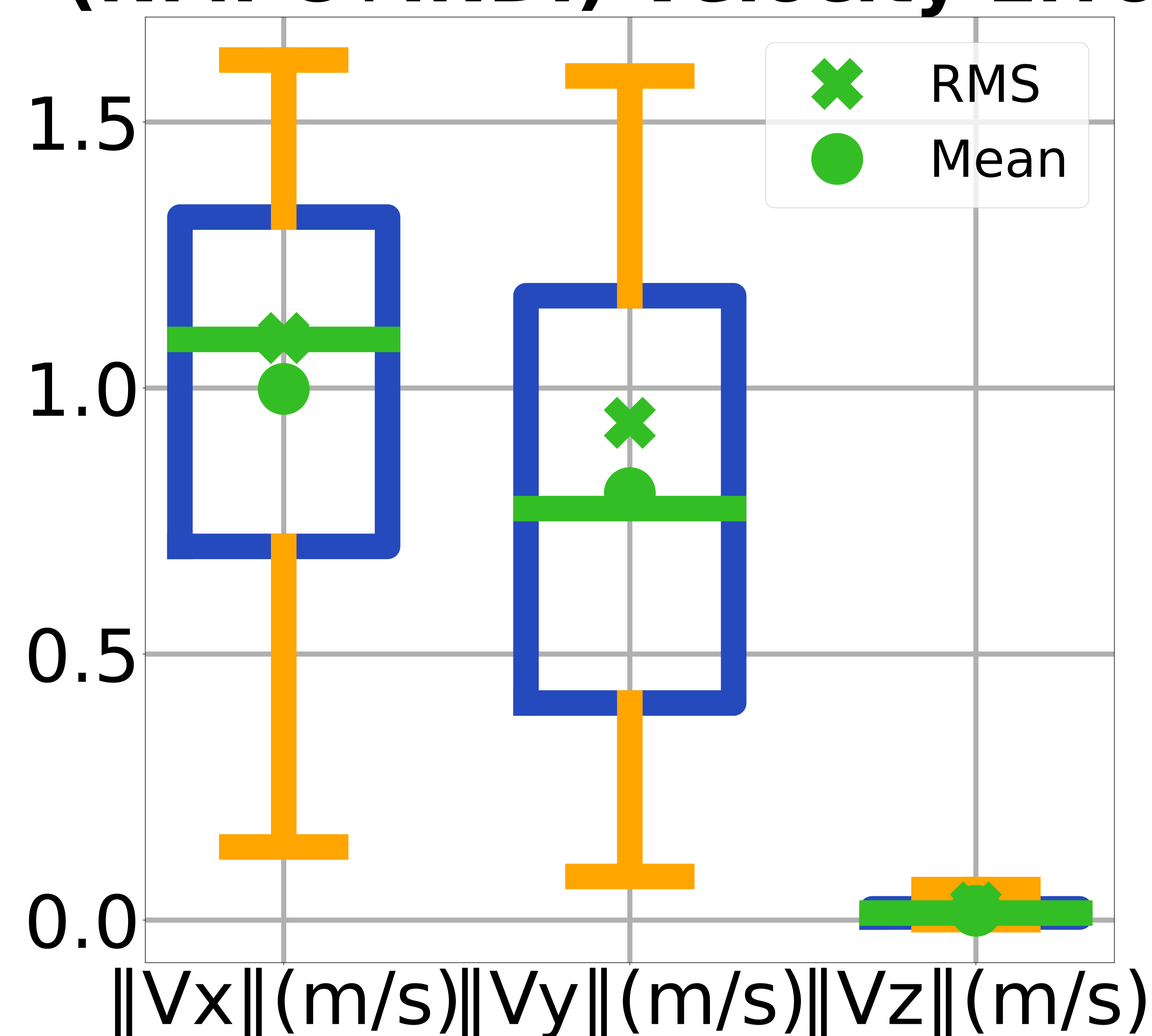
Short-1.0m/s-Fan (DFBC+INDI)-Velocity Error
