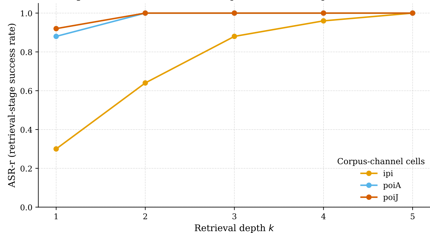
Figure F3 - ASR-r vs retrieval depth (95% bootstrap CI over seeds)
