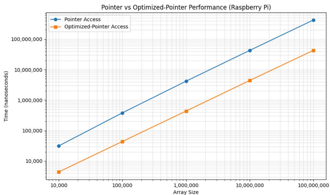
Figure 6. Raspberry Pi timing comparison of pointer-based vs manually optimized pointer-based array clearing functions of compiler-generated code with no optimization flags.
