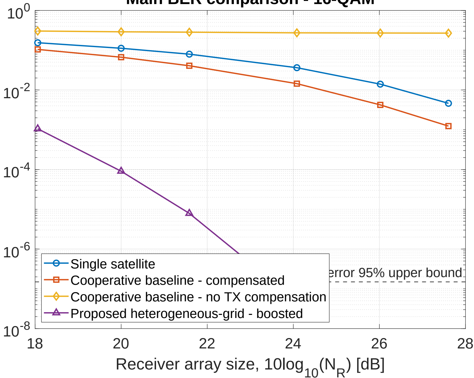
Main BER comparison - 16-QAM
