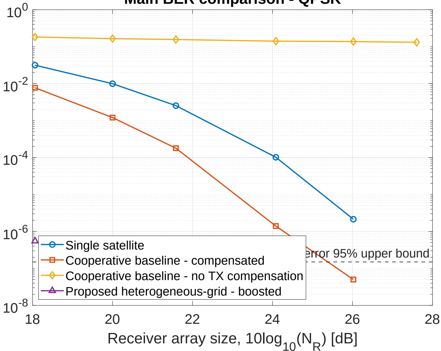
Main BER comparison - QPSK
