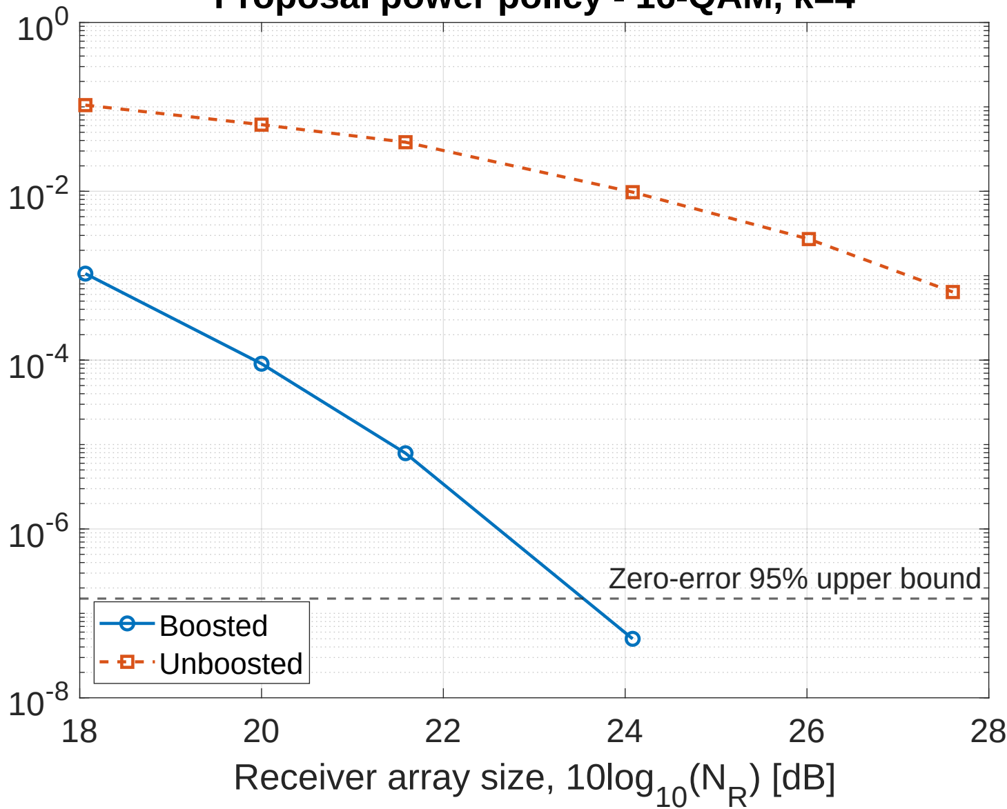
Proposal powerpolicy - 16-QAM, k=4
