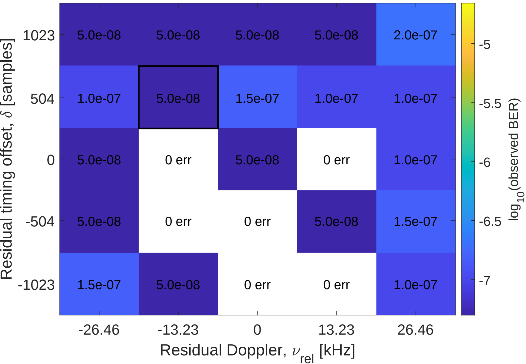
16-QAM - joint timing-Doppler sensitivity, N_R=256
