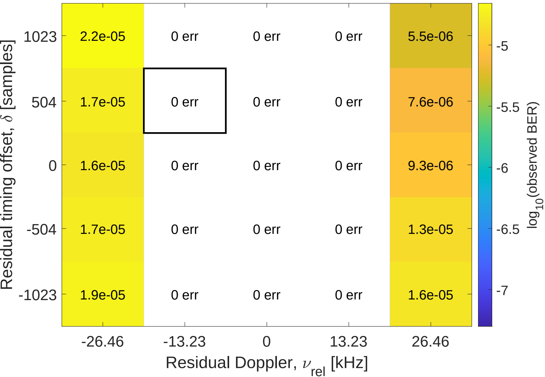
QPSK - joint timing-Doppler sensitivity, N_R=256
