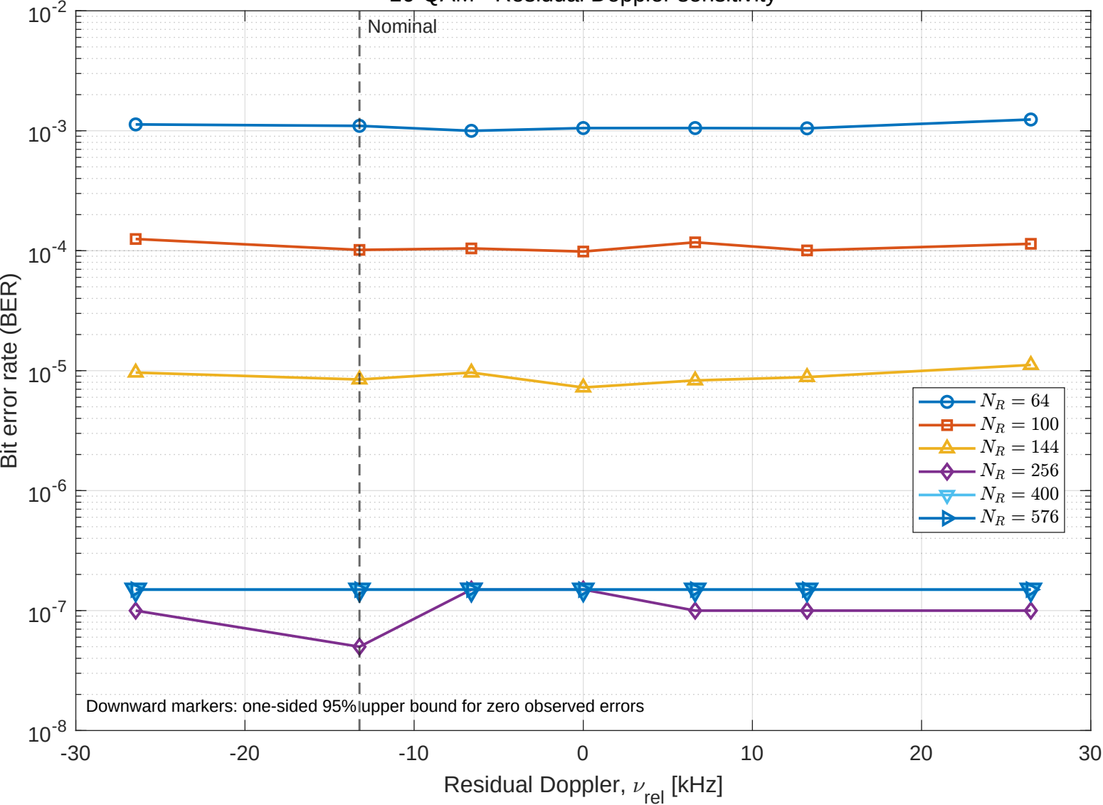
16-QAM - Residual Doppler sensitivity
