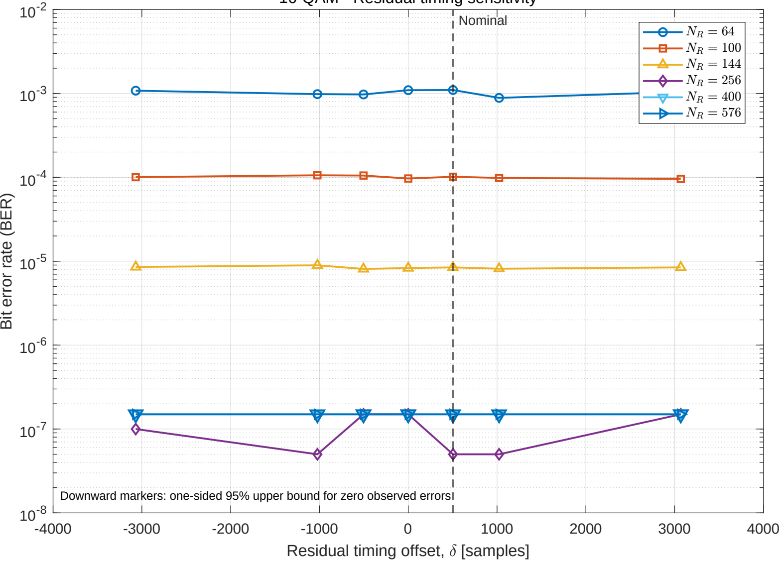
16-QAM - Residual timing sensitivity
