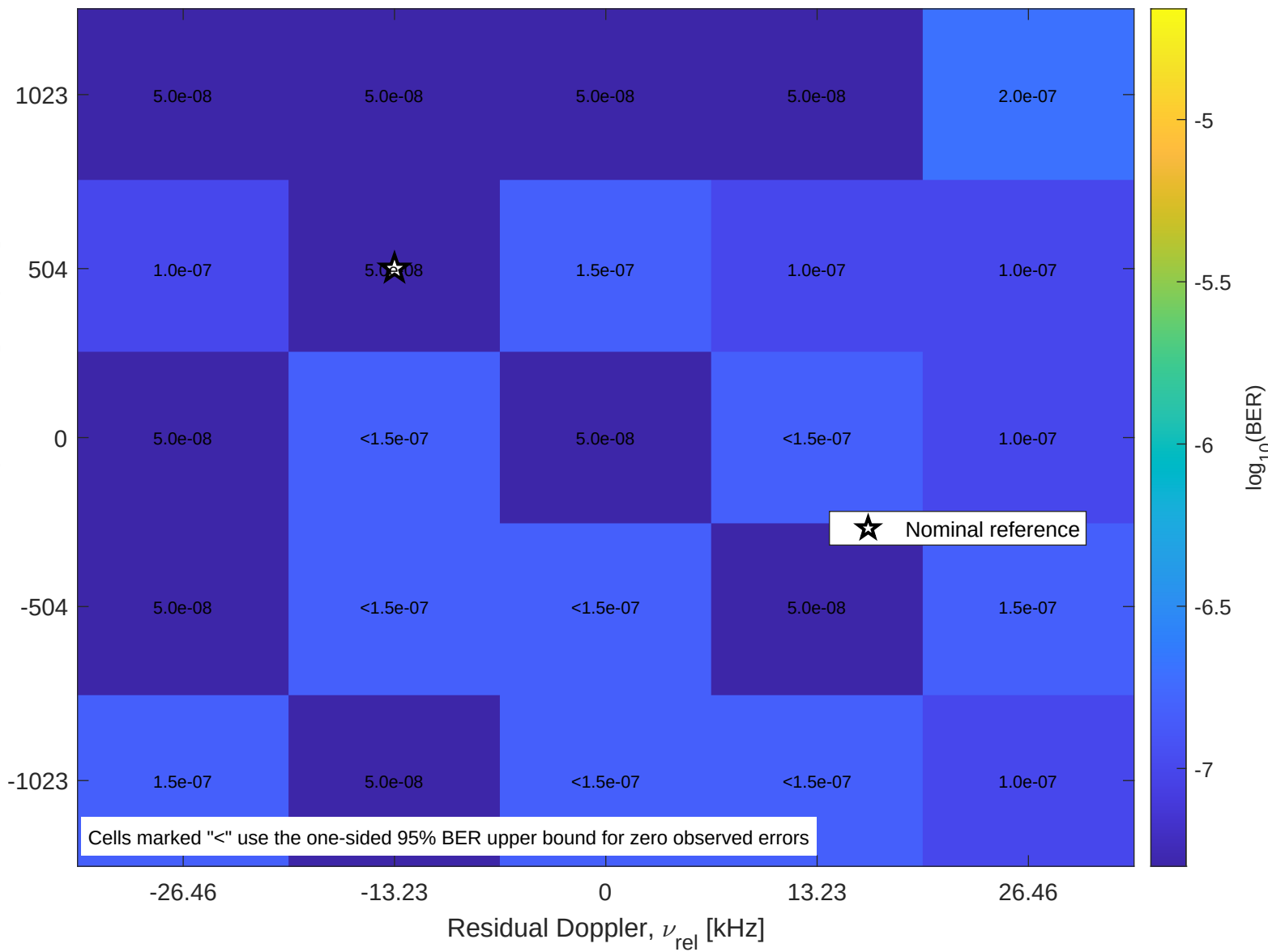
16-QAM - joint timing-Doppler sensitivity, N_R=256
