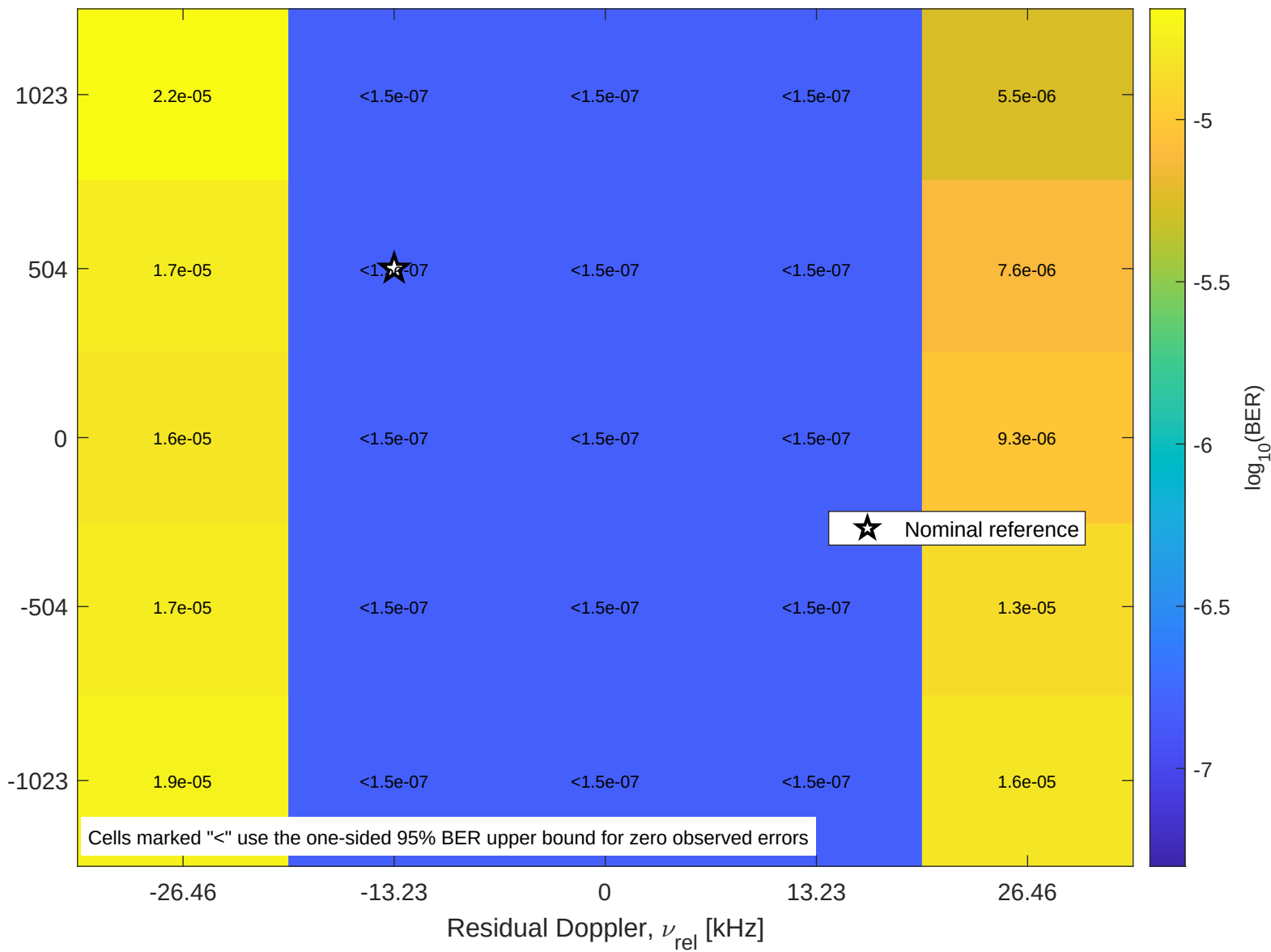
QPSK - joint timing-Doppler sensitivity, N_R=256
