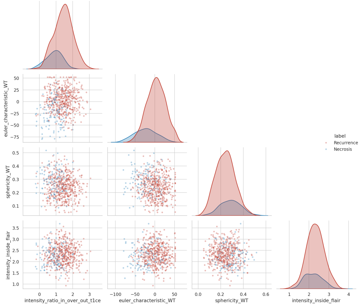
Figure 2: Pairwise exploratory feature space. The (T1ce \text{ ratio}, \chi) panel dominates separability; sphericity and FLAIR-derived intensity carry secondary subgroup structure that the anatomy prior is asked to recover.
