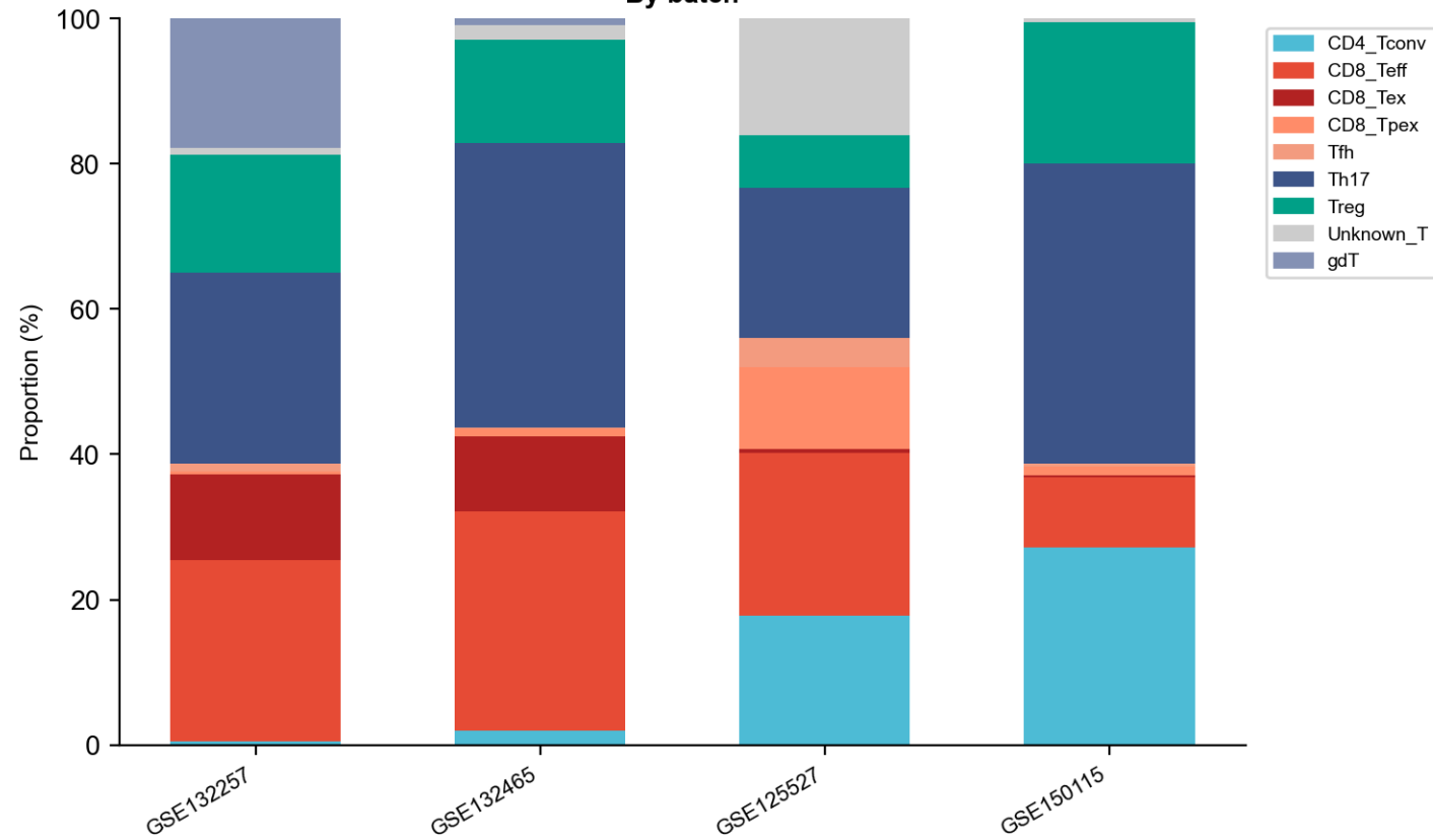
By batch
