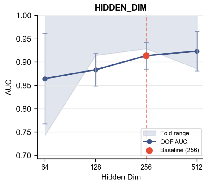
Supplementary Figure 3 — ABMIL Hyperparameter Robustness GSE178341 Immune Microenvironment · 5-Fold CV OOF AUC
