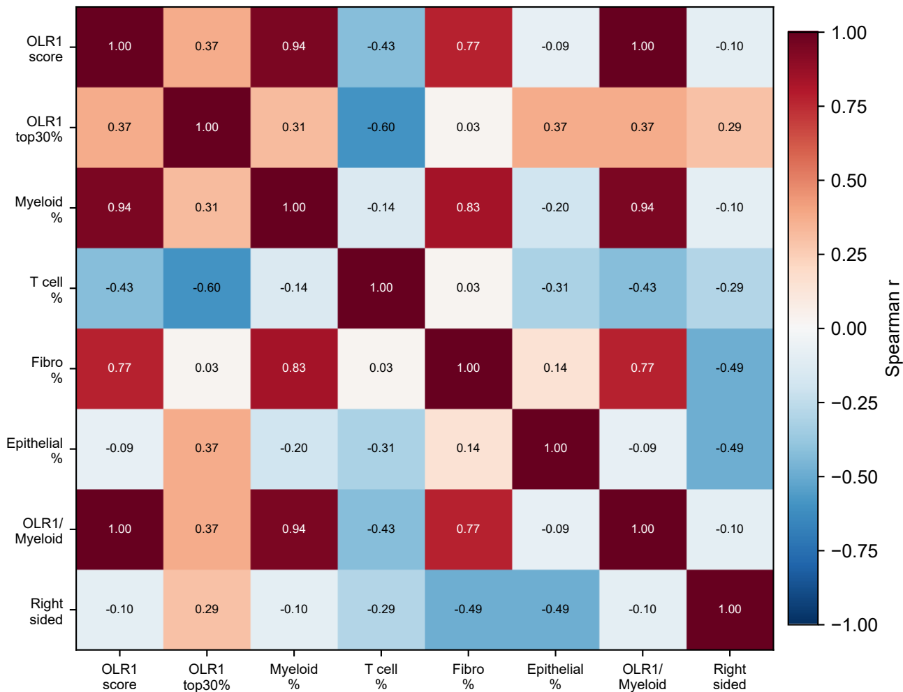
E OLR1+ TAM Abundance vs TME Composition (per-sample Spearman, n=6, GSE188711)
