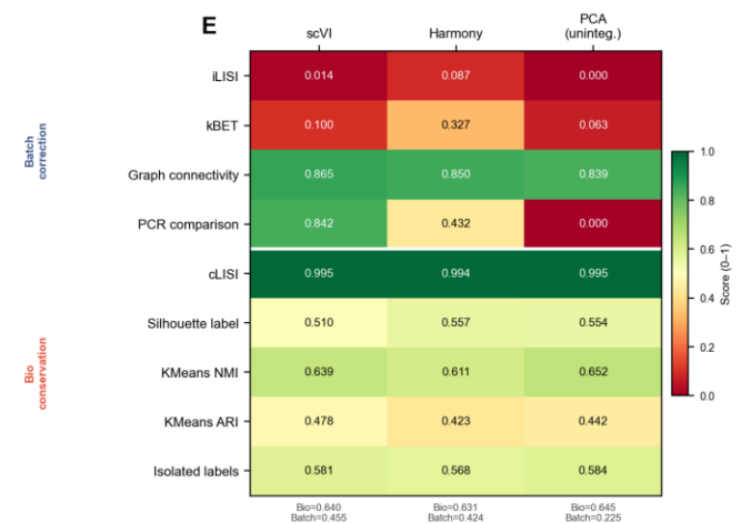
Integration Quality (scib-metrics)
