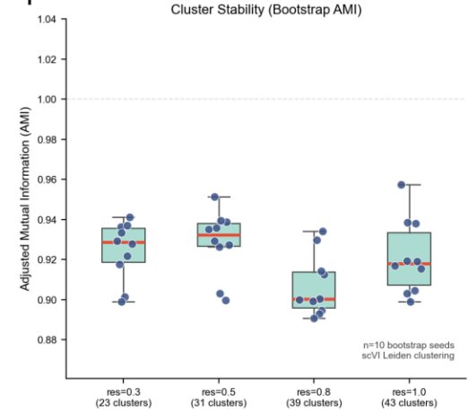
Cluster Stability (Bootstrap AMI)
