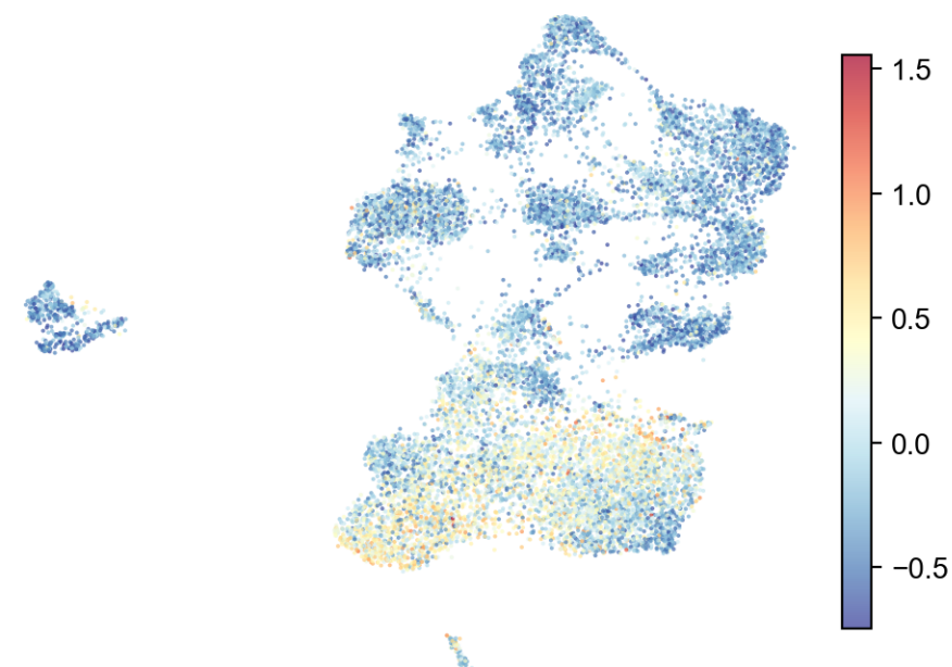
MYC ( \rho=+0.11 )
