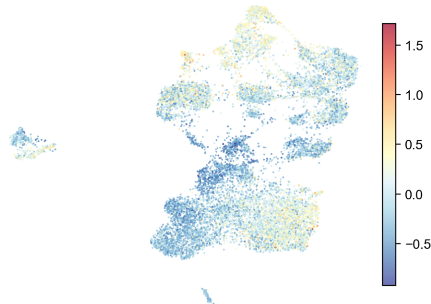
NFKB1 ( \rho=+0.12 )
