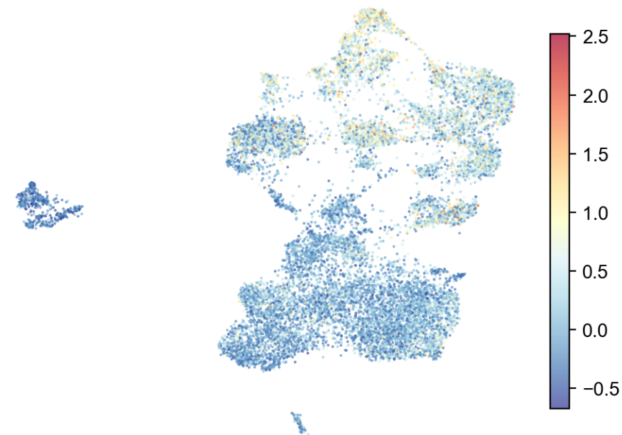
MYC ( \rho=+0.11 )
