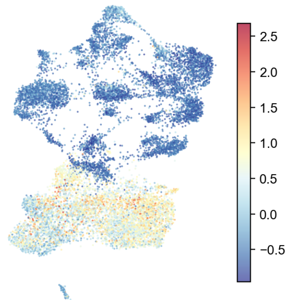
KLF4 ( \rho=-0.16 )
