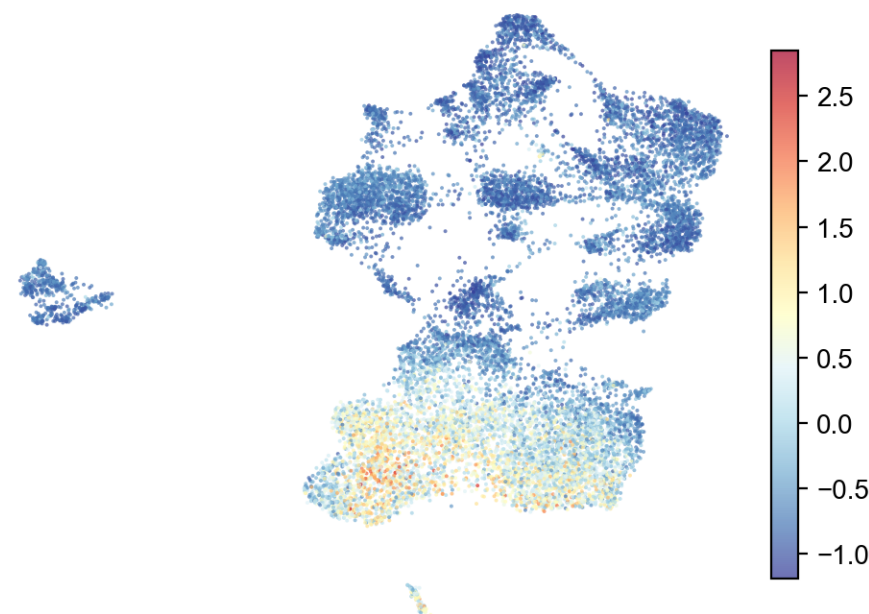
NFKB1 ( \rho=+0.12 )
