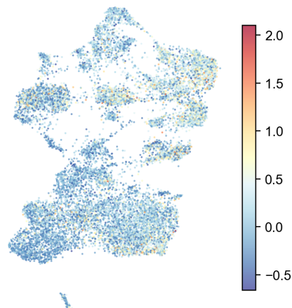
KLF4 ( \rho=-0.16 )
