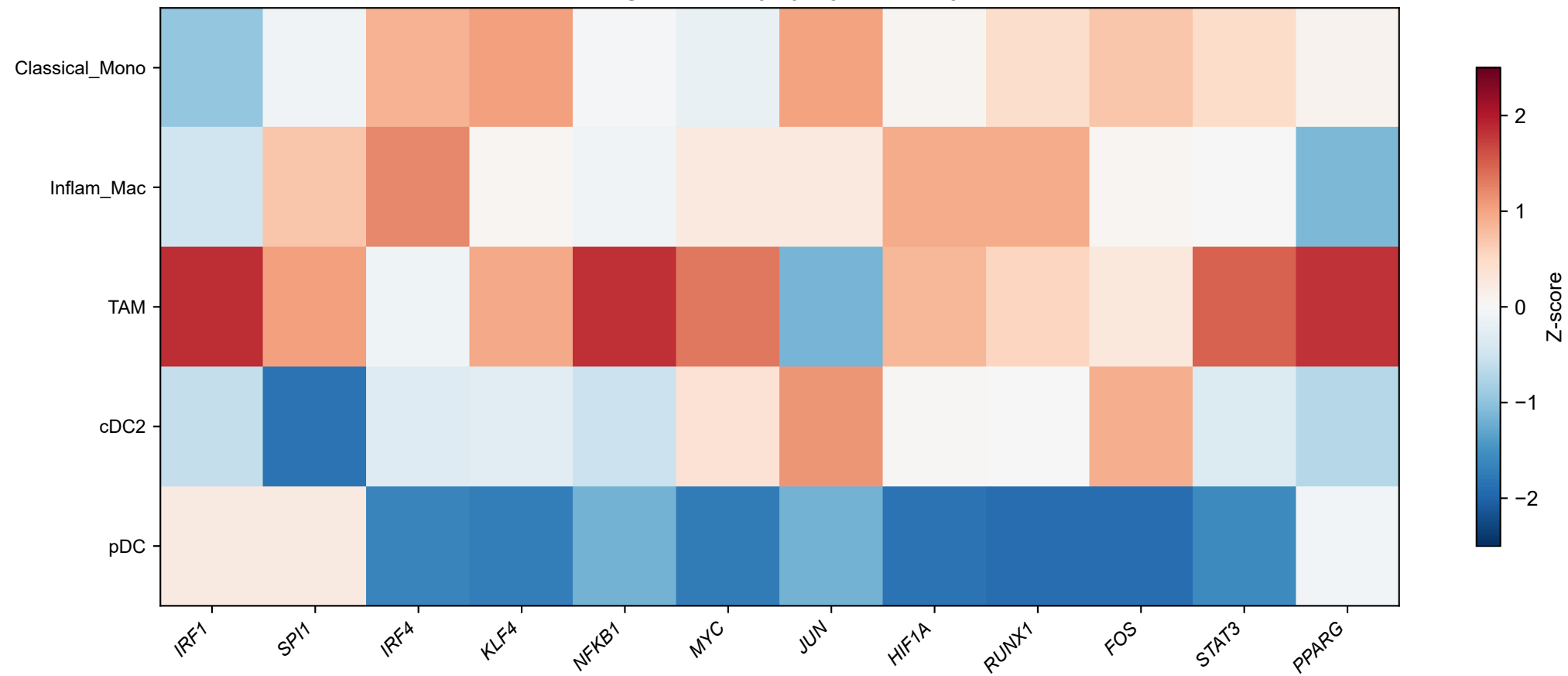
TF regulon activity by myeloid subtype
