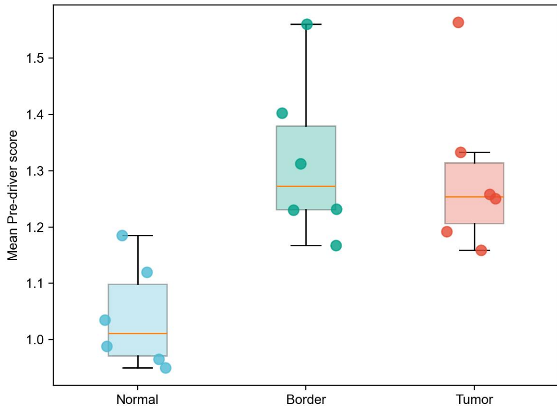
Mean Pre-driver score
