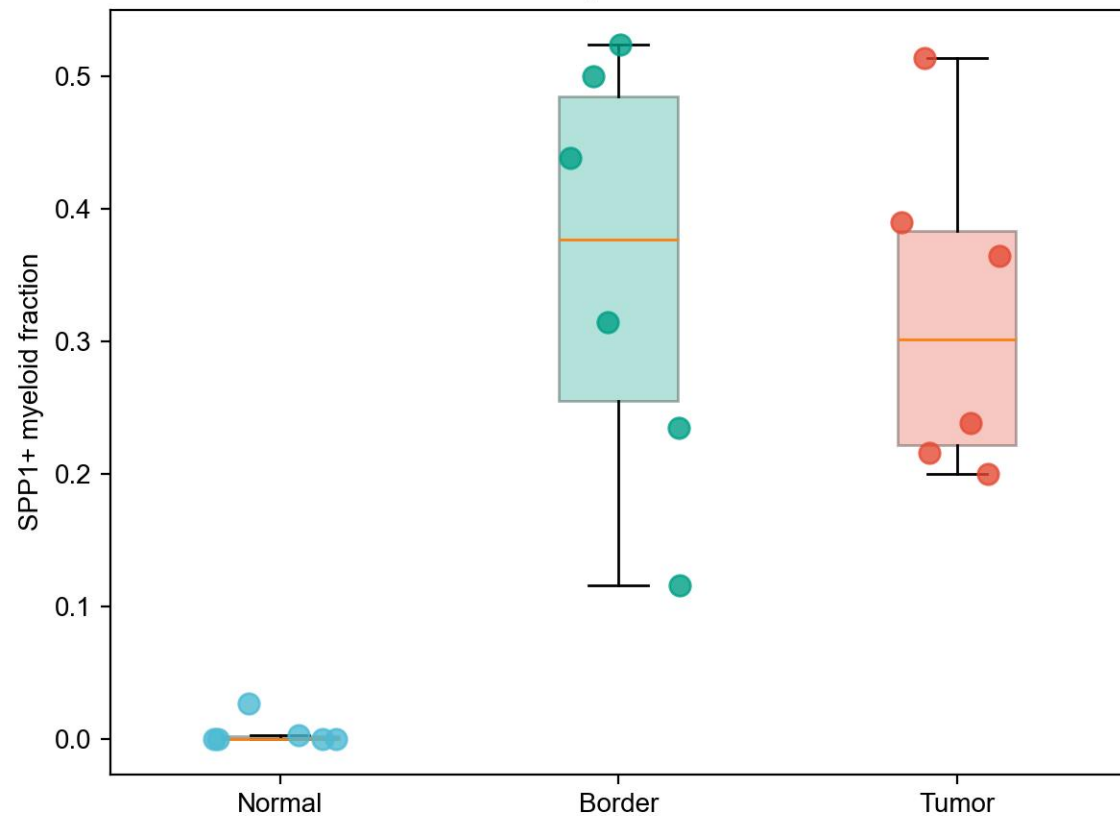
SPP1+ myeloid fraction
