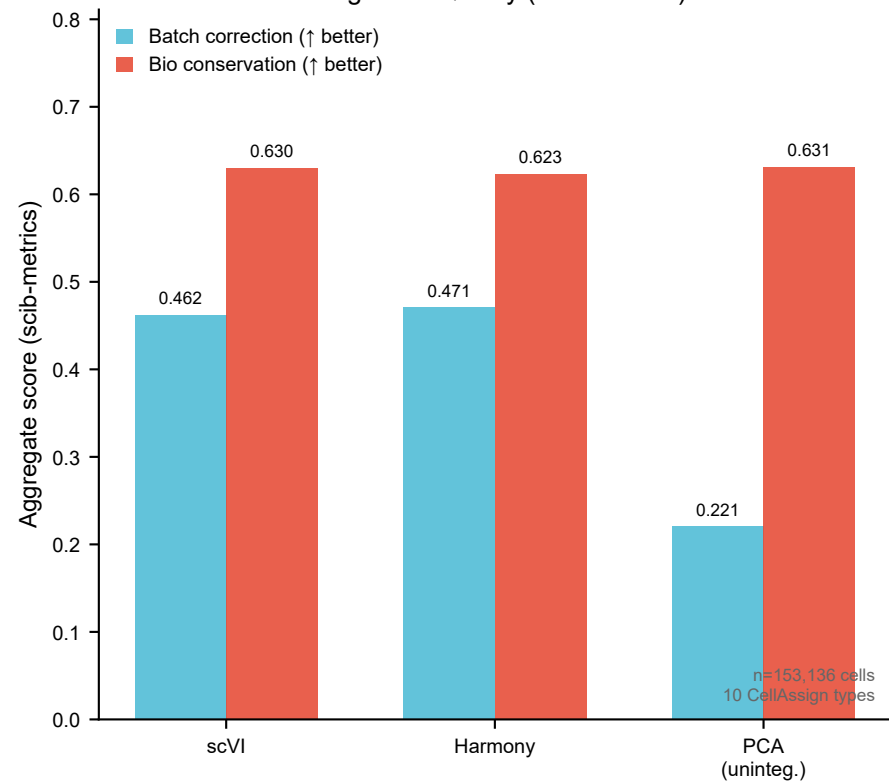
F Integration Quality (scib-metrics)
