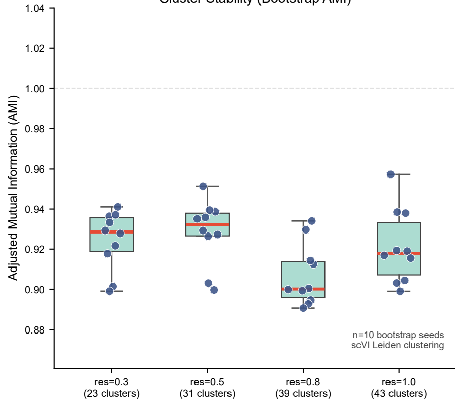
Cluster Stability (Bootstrap AMI)
