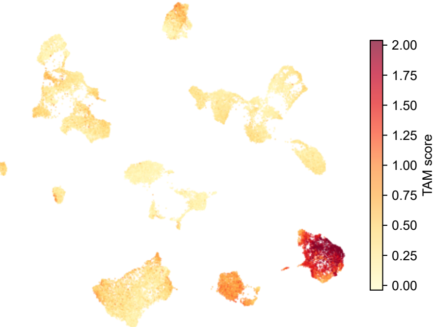
TAM Signature Score
