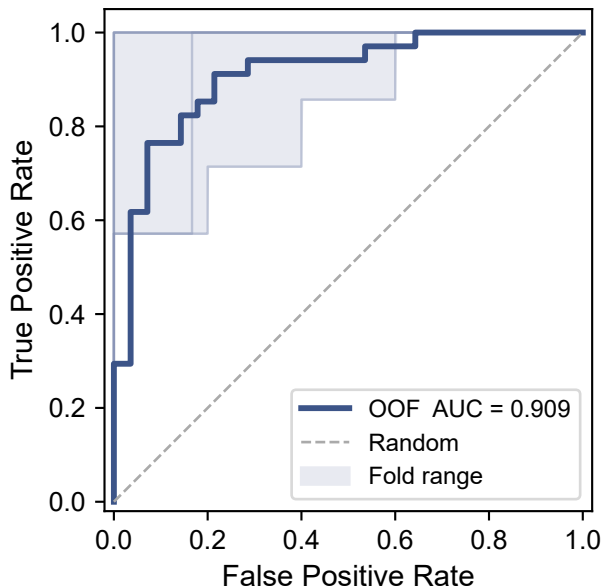
ROC Curve
