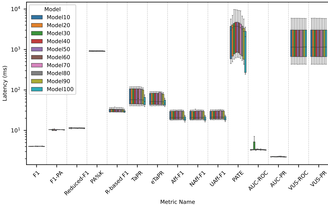
Latency Distribution by Model for TS Length 10k
