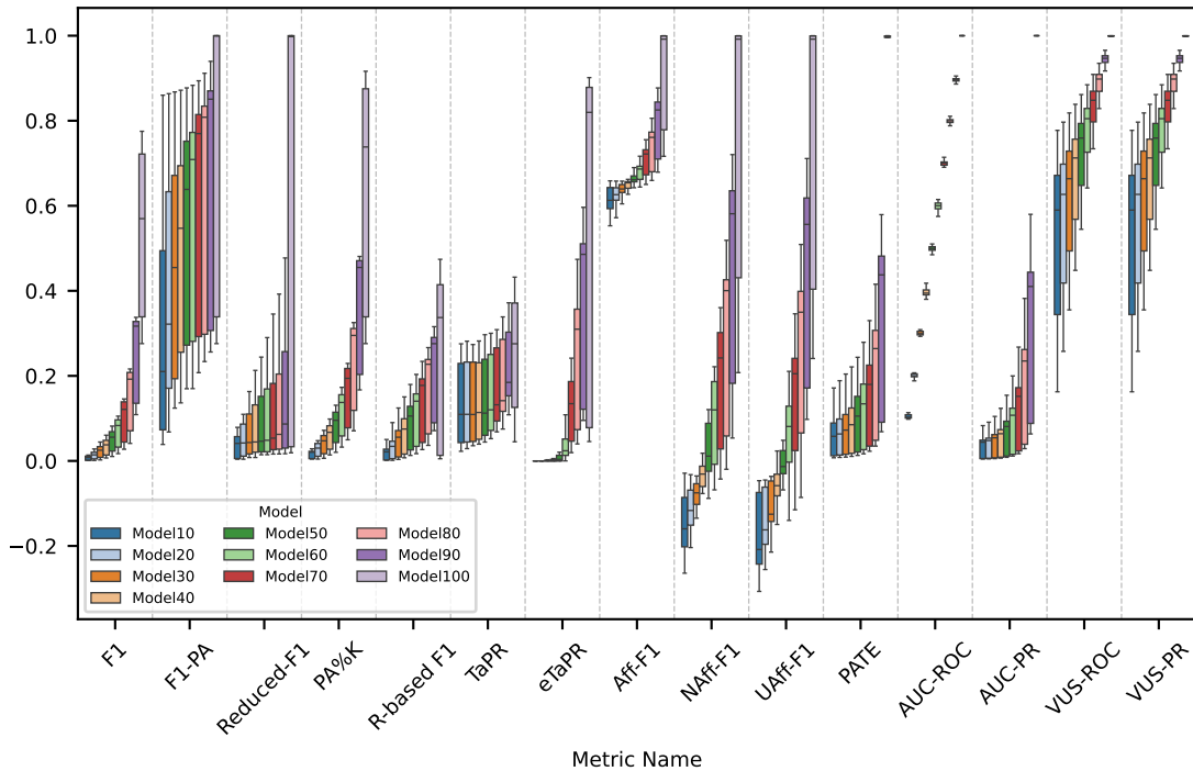
Metric Score Distribution by Model for TS Length 10k
