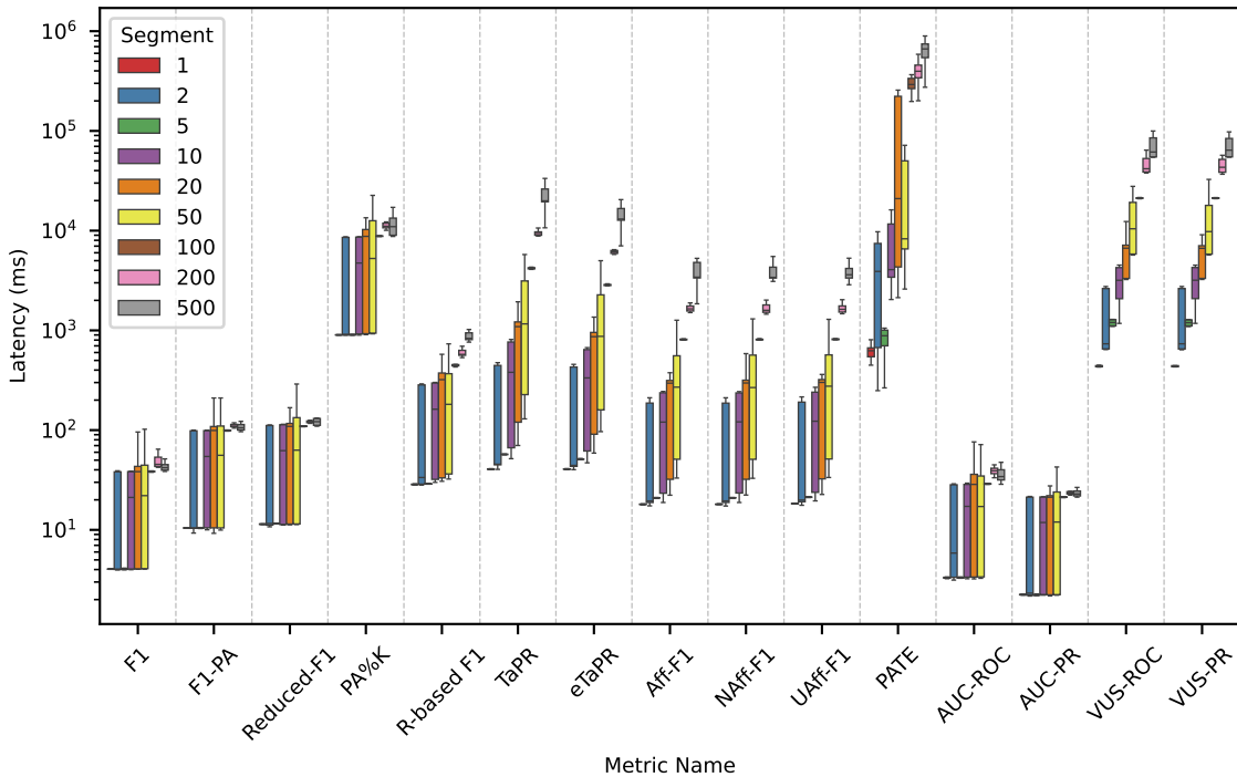
Latency Distribution Across Different Segment Counts
