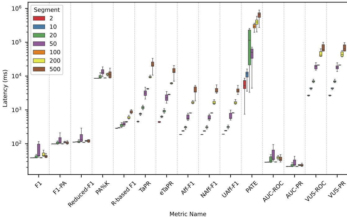
Latency Distribution with TS Length 100k Across Different Segment Counts
