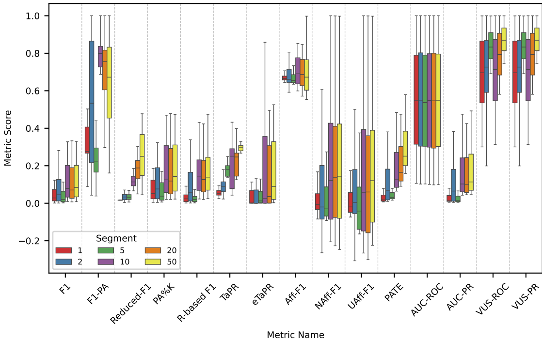
Metric Score Distribution with TS Length 10k Across Different Segment Counts
