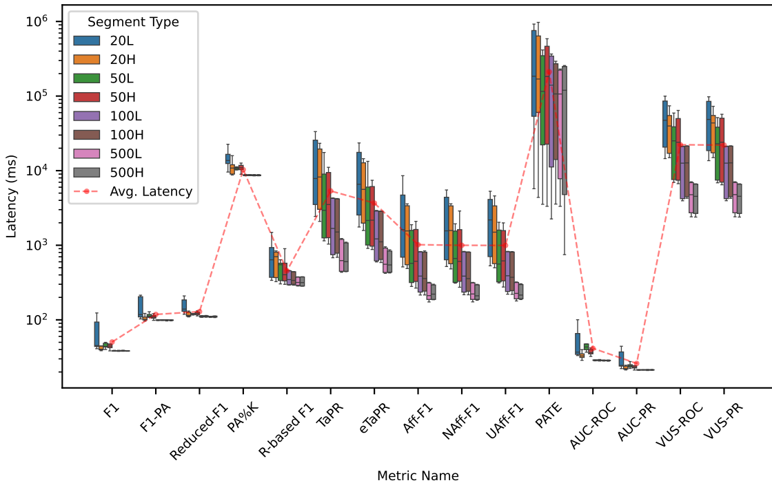
Latency Distribution for TS Length = 100k
