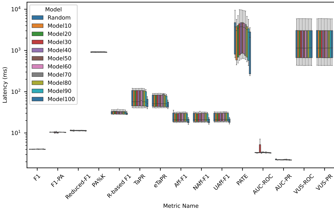
Latency Distribution for TS Length = 10k
