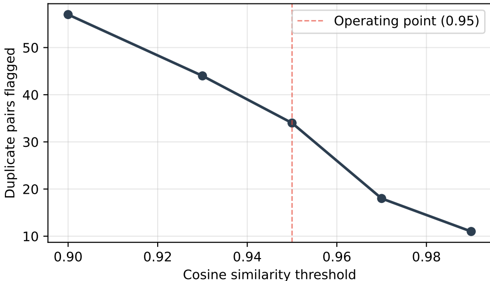
Deduplication threshold sensitivity
