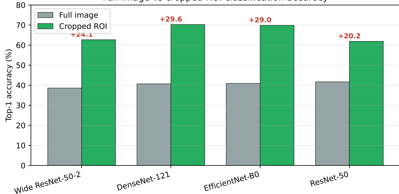
Full image vs cropped ROI classification accuracy
