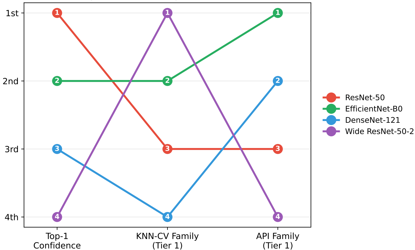
Model ranking under three independent validation channels
